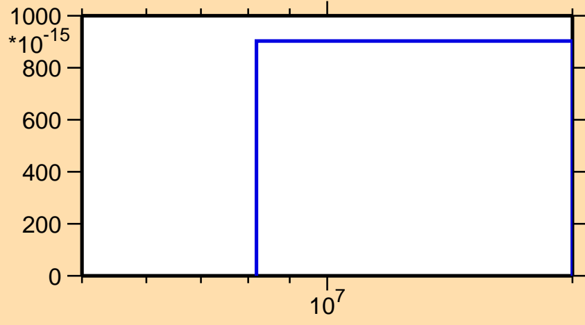
\sigma vs. E for ^{125}\text{In}(n,nd)
