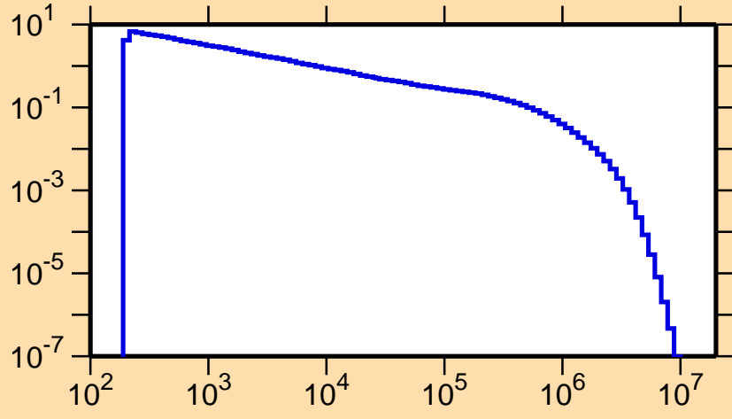
\sigma vs. E for ^{196}\text{Ir}(n,n_2)
