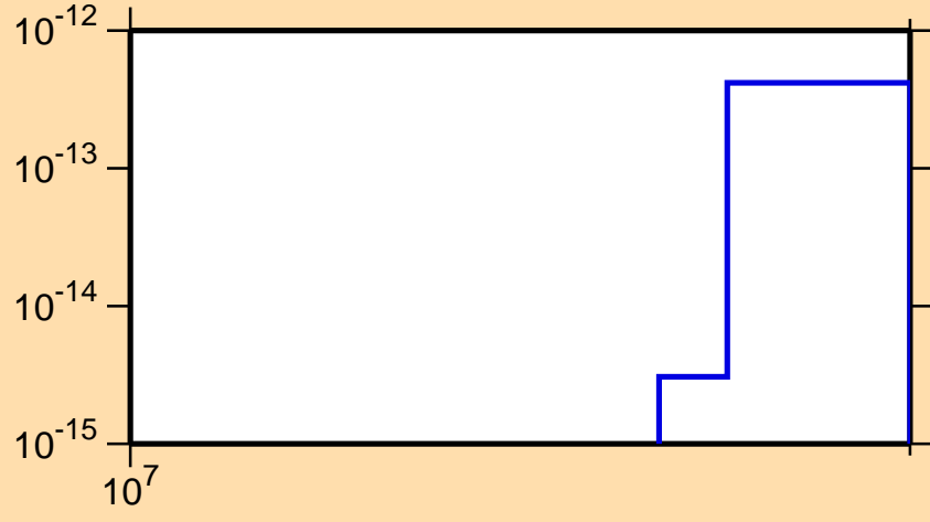
\sigma vs. E for ^{196}\text{Ir}(n,\text{He}3)
