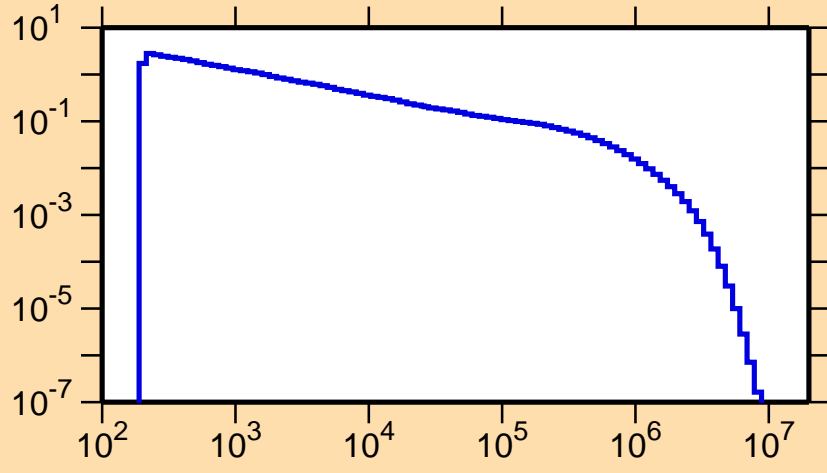
\sigma vs. E for ^{196}\text{Ir}(n,n_1)
