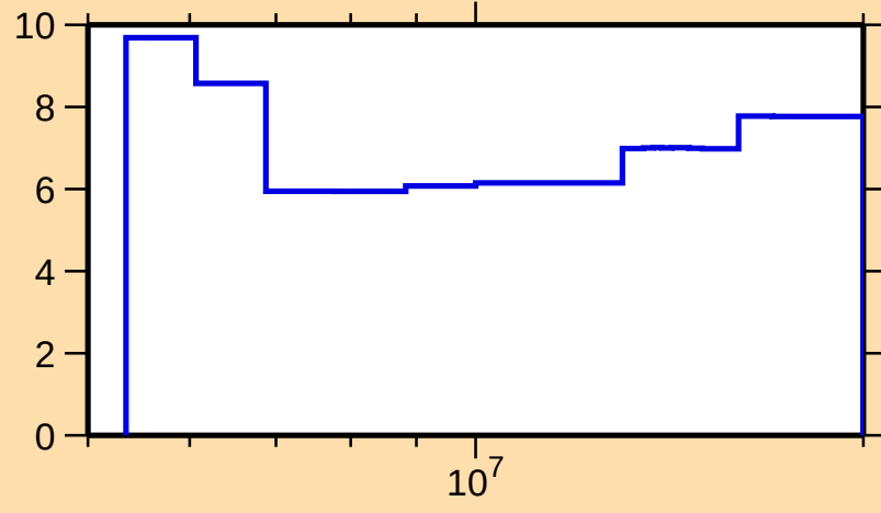
\Delta\sigma/\sigma vs. E for ^{73}\text{Kr}(\text{n},\text{nonel.})
