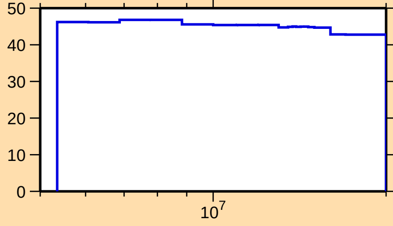
\Delta\sigma/\sigma vs. E for ^{73}\text{Kr}(\text{n},\text{inel.})
