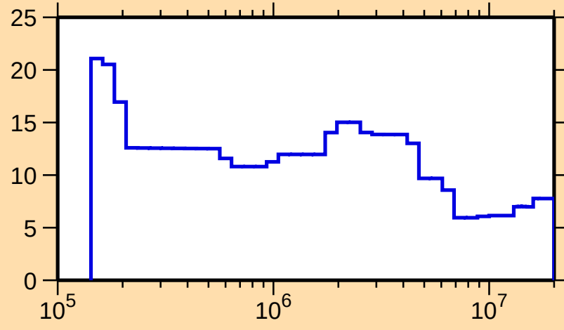
\Delta\sigma/\sigma vs. E for ^{73}\text{Kr}(\text{n,nonel.})
