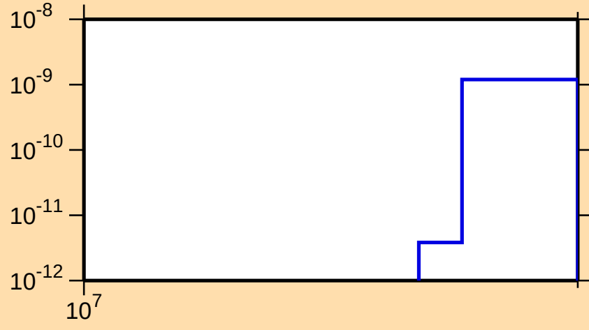
\sigma vs. E for ^{73}\text{Kr}(n,2n\alpha)
