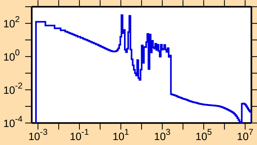
\sigma vs. E for ^{73}\text{Kr}(n,\gamma)
