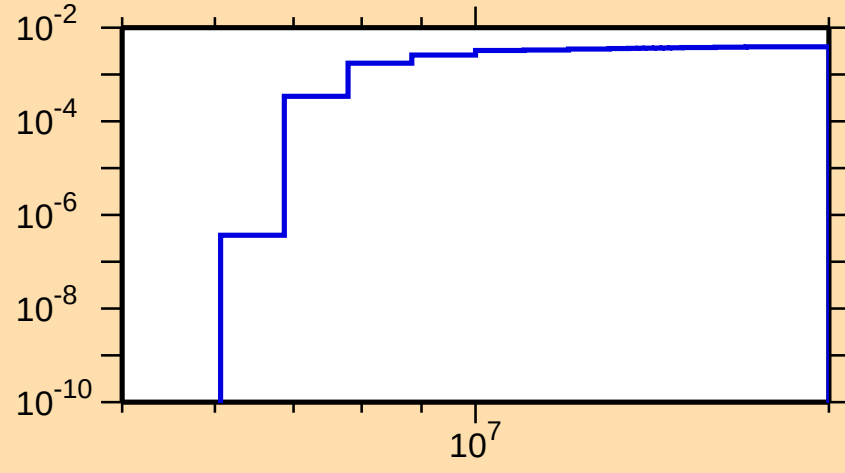
\sigma vs. E for ^{73}\text{Kr}(n,n\text{cont.})
