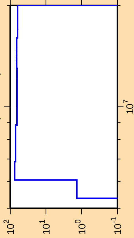
\Delta\sigma/\sigma vs. E for ^{73}\text{Kr}(\text{n},\text{ncont.})
