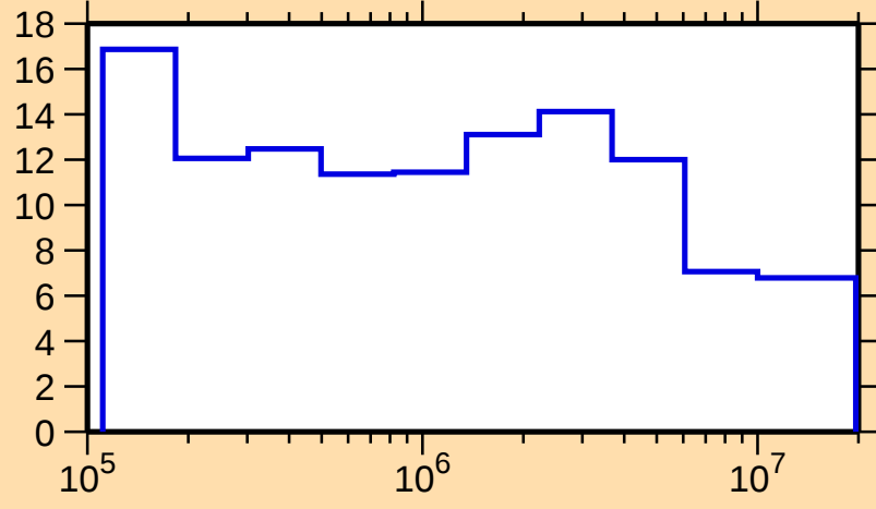
\Delta\sigma/\sigma vs. E for ^{73}\text{Kr}(\text{n,nonel.})
