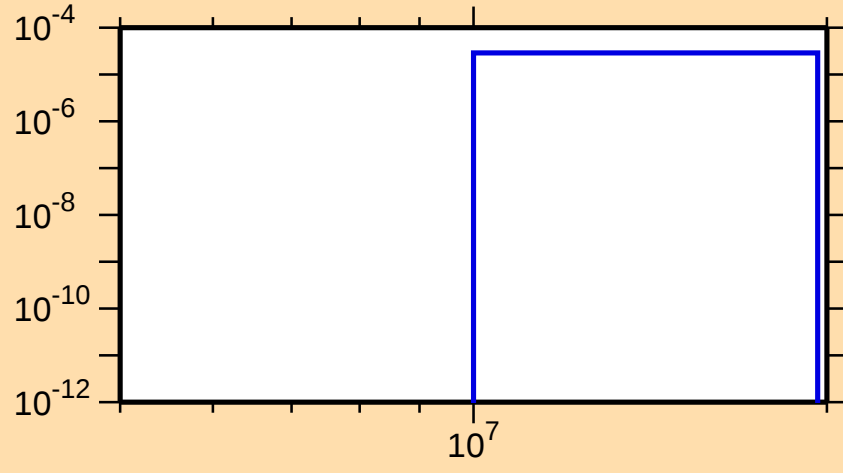
\sigma vs. E for ^{73}\text{Kr}(n,\text{pt})
