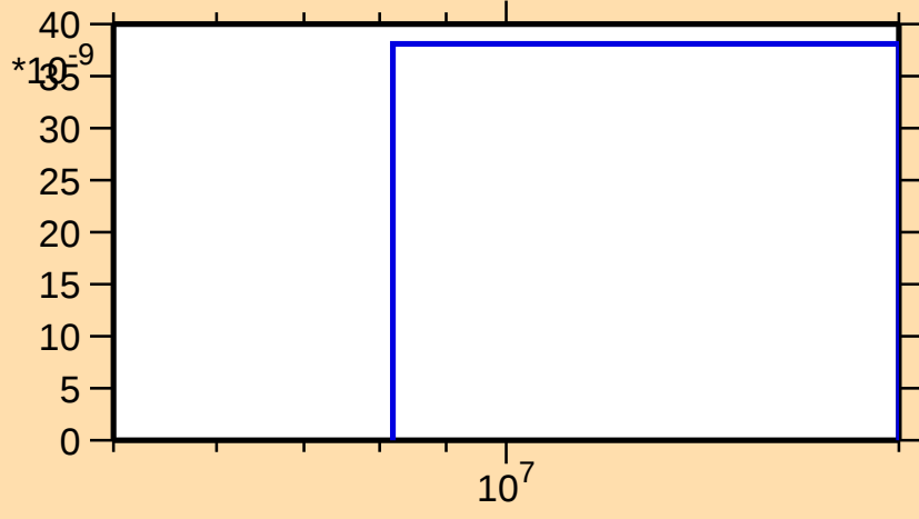
\sigma vs. E for ^{73}\text{Kr}(n,nd)
