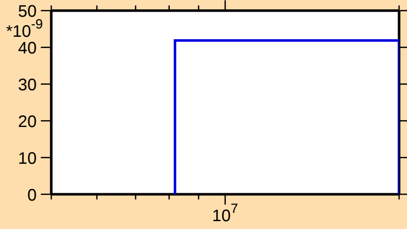
\sigma vs. E for ^{73}\text{Kr}(\text{mt117})
