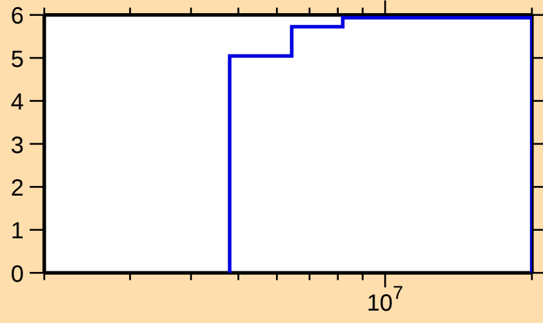
\Delta\sigma/\sigma vs. E for ^{73}\text{Kr}(\text{n},\text{tot.})
