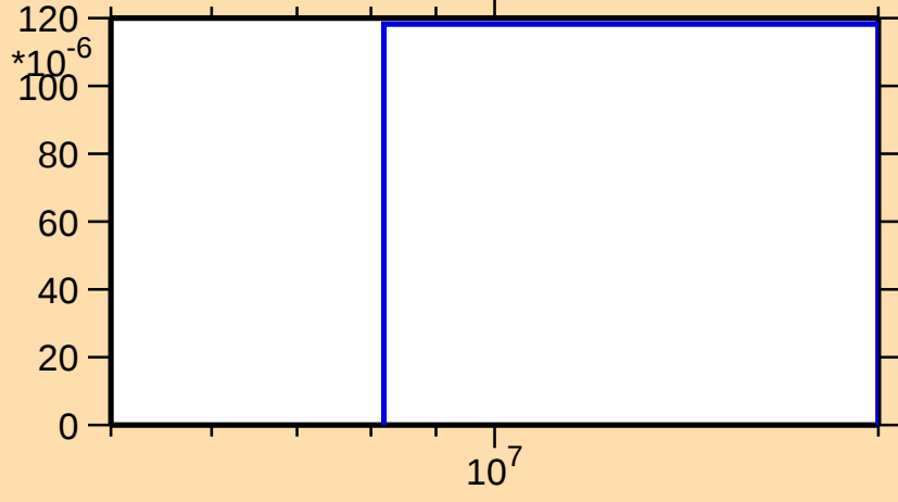
\sigma vs. E for ^{73}\text{Kr}(n,2n)
