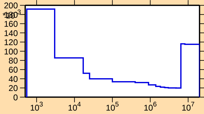
\sigma vs. E for ^{73}\text{Kr}(n,\alpha)
