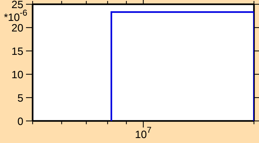
\sigma vs. E for ^{73}\text{Kr}(n,\text{pt})
