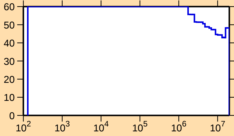
\Delta\sigma/\sigma vs. E for ^{81}\text{Kr}(n,p)
