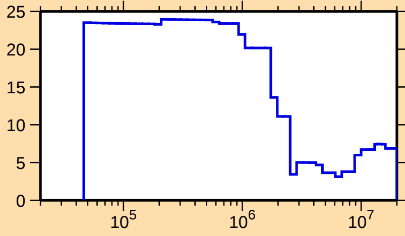
\Delta\sigma/\sigma vs. E for ^{81}\text{Kr}(n,\text{tot.})
