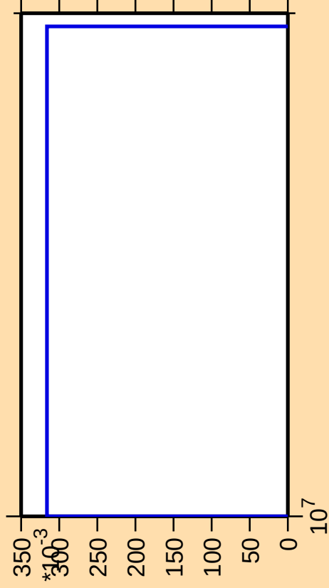
\Delta\sigma/\sigma vs. E for ^{81}\text{Kr}(n,3n)
