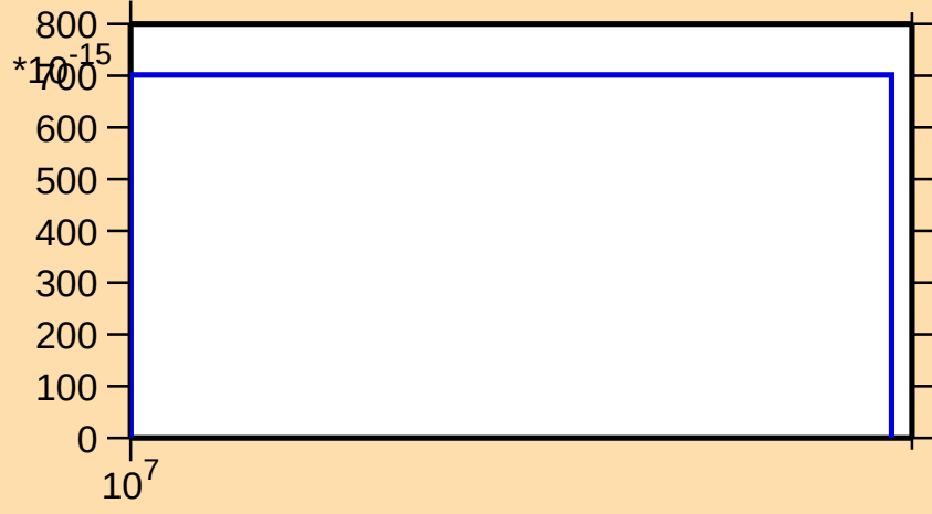
\sigma vs. E for ^{81}\text{Kr}(n,3n)
