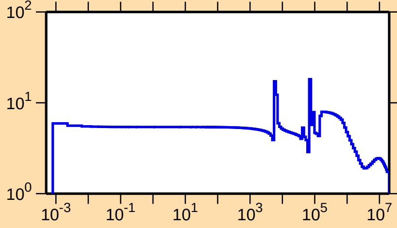
\sigma vs. E for ^{90}\text{Kr}(n,\text{el.})
