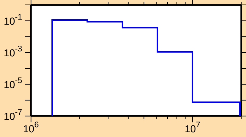
\sigma vs. E for ^{90}\text{Kr}(n,n_2)
