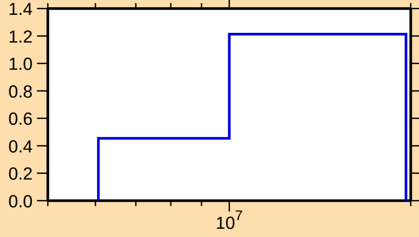
\sigma vs. E for ^{90}\text{Kr}(n,2n)
