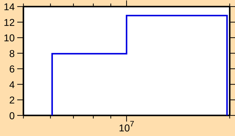
\Delta\sigma/\sigma vs. E for ^{90}\text{Kr}(n,\text{tot.})
