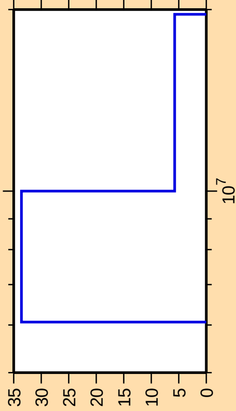
\Delta\sigma/\sigma vs. E for ^{90}\text{Kr}(n,2n)
