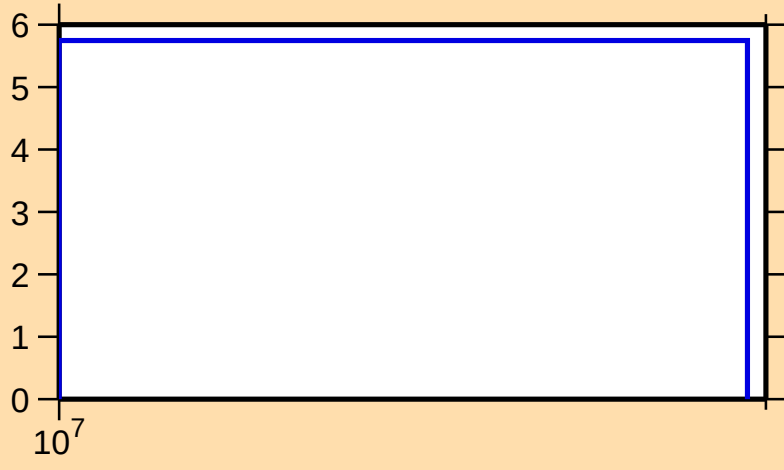
\Delta\sigma/\sigma vs. E for ^{90}\text{Kr}(n,2n)
