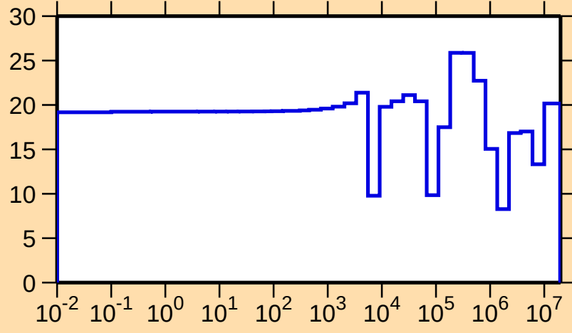
\Delta\sigma/\sigma vs. E for ^{90}\text{Kr}(n,\text{el.})
