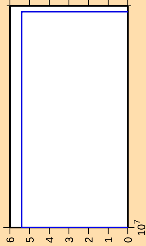
\Delta\sigma/\sigma vs. E for ^{90}\text{Kr}(n,\text{nd})
