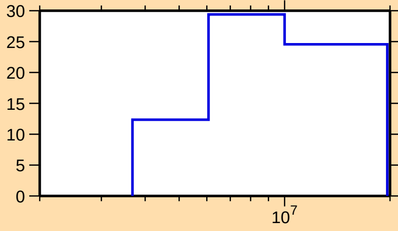
\Delta\sigma/\sigma vs. E for ^{90}\text{Kr}(\text{n},\text{inel.})
