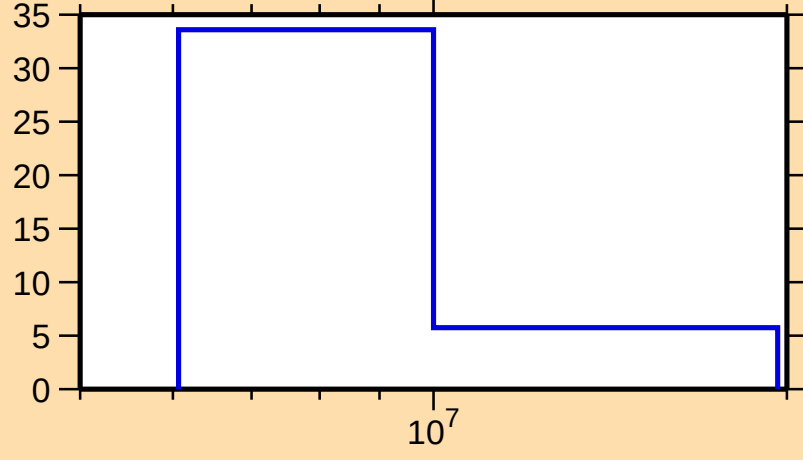
\Delta\sigma/\sigma vs. E for ^{90}\text{Kr}(n,2n)
