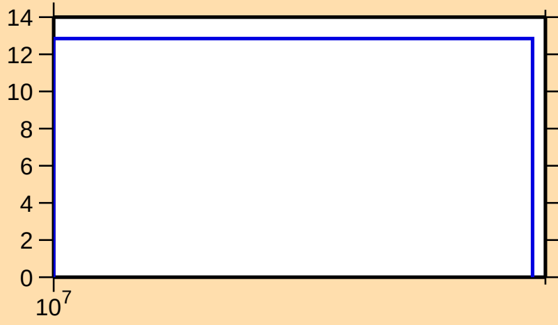
\Delta\sigma/\sigma vs. E for ^{90}\text{Kr}(n,\text{tot.})
