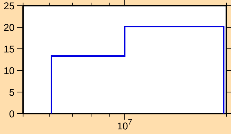
\Delta\sigma/\sigma vs. E for ^{90}\text{Kr}(n,\text{el.})
