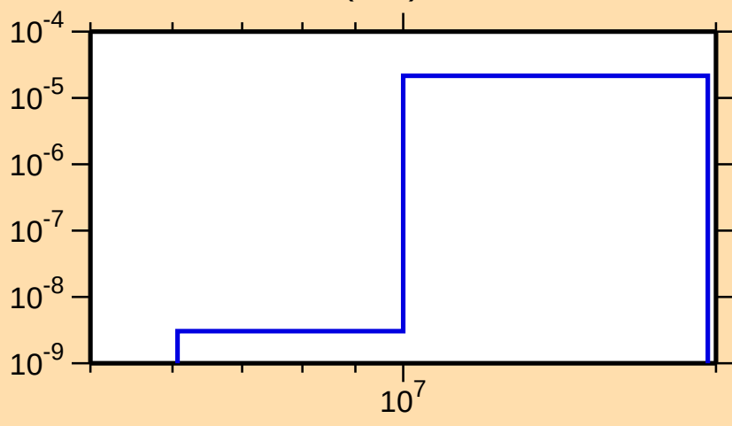
\sigma vs. E for ^{90}\text{Kr}(n,\alpha)
