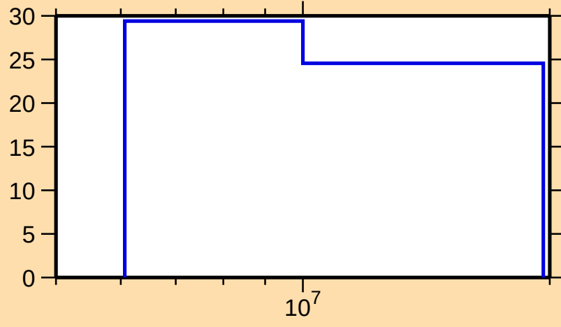
\Delta\sigma/\sigma vs. E for ^{90}\text{Kr}(n,\text{inel.})
