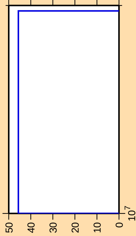
\Delta\sigma/\sigma vs. E for ^{90}\text{Kr}(n,3n)
