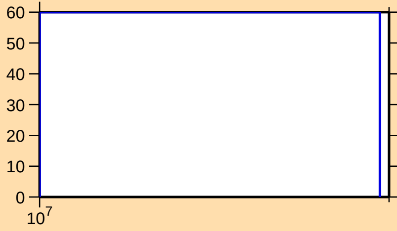
\Delta\sigma/\sigma vs. E for ^{90}\text{Kr}(n,p)
