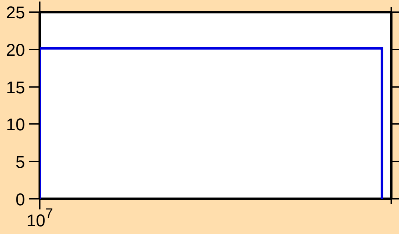
\Delta\sigma/\sigma vs. E for ^{90}\text{Kr}(\text{n,el.})
