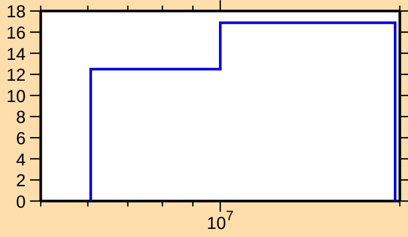
\Delta\sigma/\sigma vs. E for ^{90}\text{Kr}(n,\text{nonel.})
