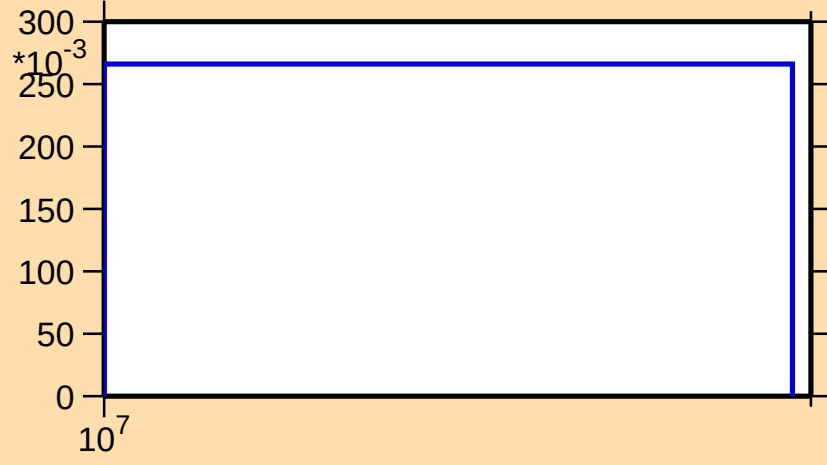
\sigma vs. E for ^{90}\text{Kr}(n,3n)
