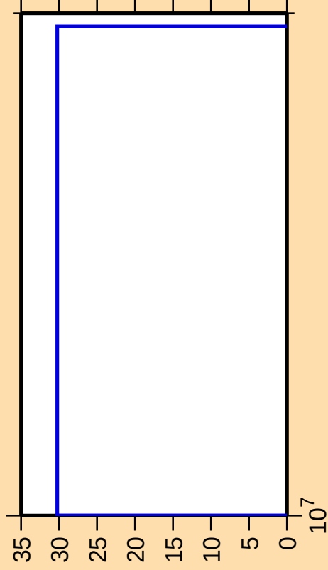
\Delta\sigma/\sigma vs. E for ^{90}\text{Kr}(n,2n\alpha)
