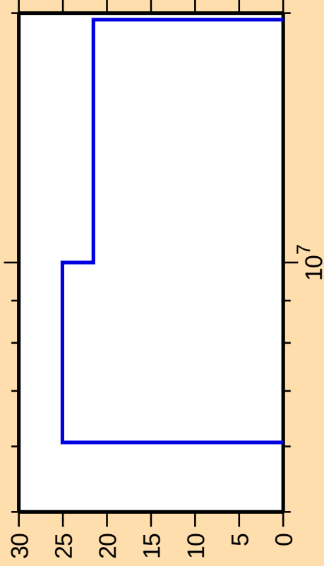
\Delta\sigma/\sigma vs. E for ^{90}\text{Kr}(n,n_1)
