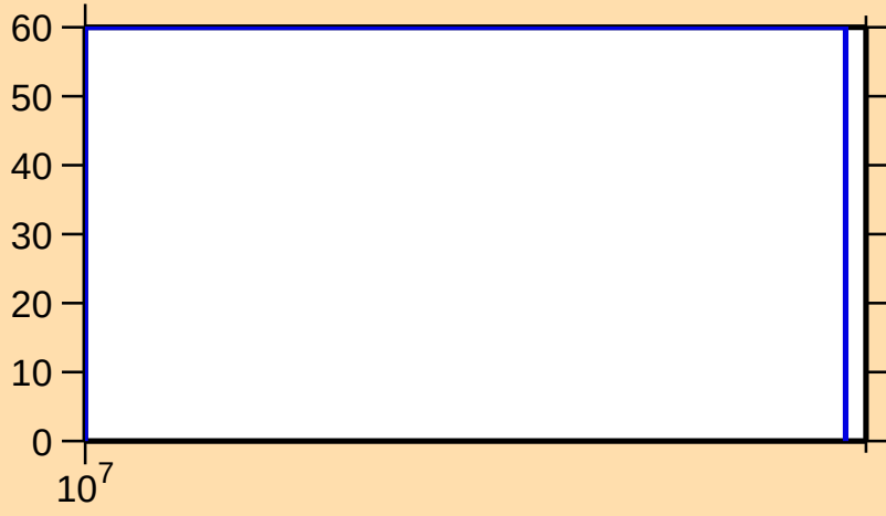
\Delta\sigma/\sigma vs. E for ^{90}\text{Kr}(n,\gamma)
