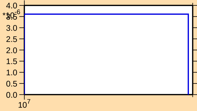
\sigma vs. E for ^{90}\text{Kr}(n,d)
