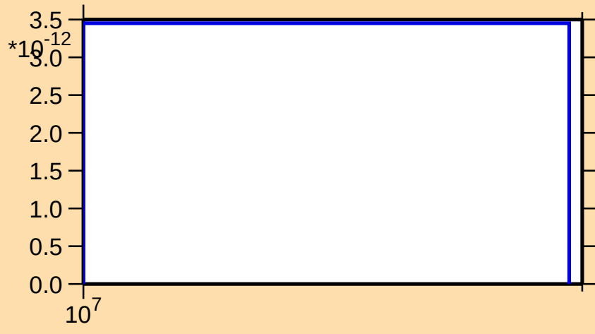
\sigma vs. E for ^{90}\text{Kr}(n,2n\alpha)
