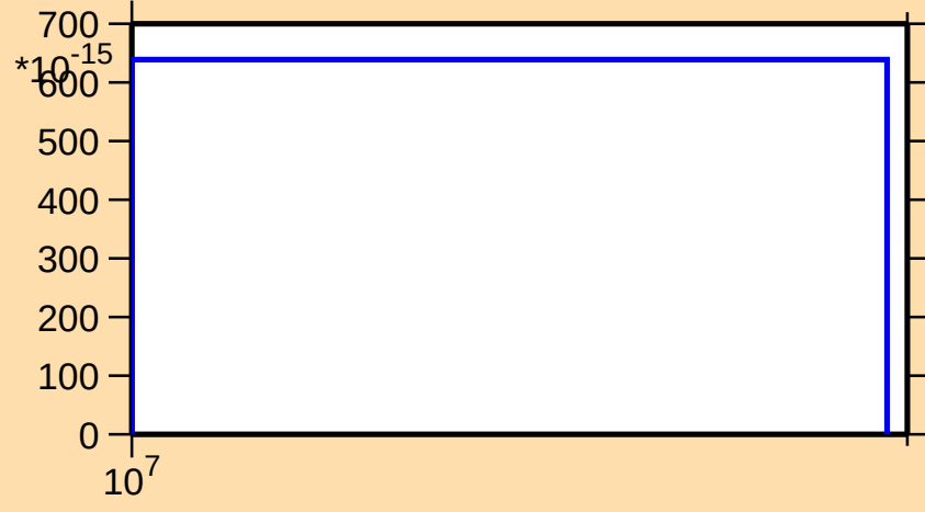
\sigma vs. E for ^{90}\text{Kr}(n,\text{nd})
