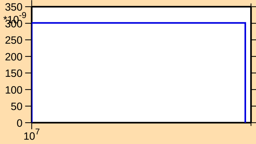
\sigma vs. E for ^{90}\text{Kr}(n,np)
