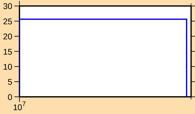
\Delta\sigma/\sigma vs. E for ^{90}\text{Kr}(n,n\text{cont.})
