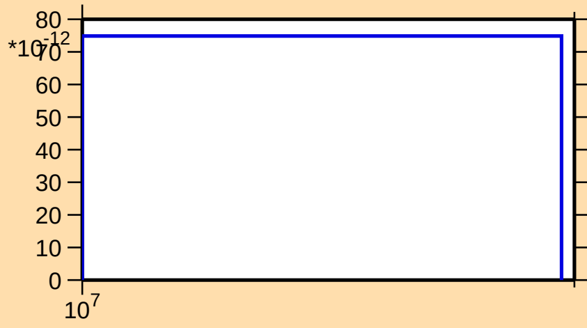
\sigma vs. E for ^{90}\text{Kr}(n,nt)
