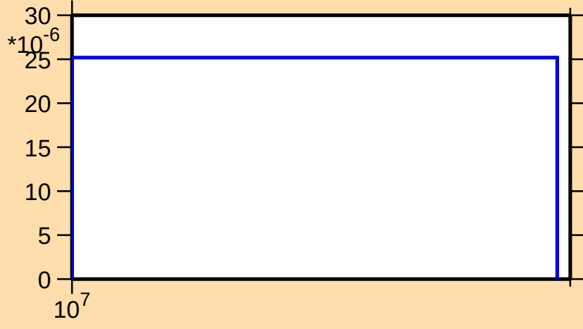
\sigma vs. E for ^{90}\text{Kr}(n,p)
