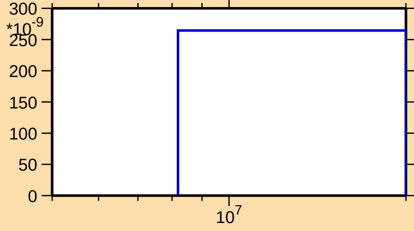
\sigma vs. E for ^{90}\text{Kr}(n,np)
