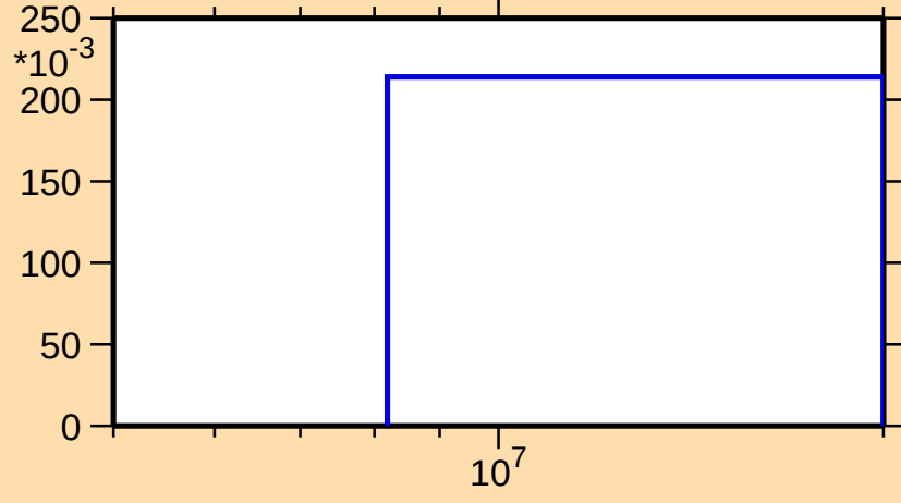
\sigma vs. E for ^{90}\text{Kr}(n,3n)
