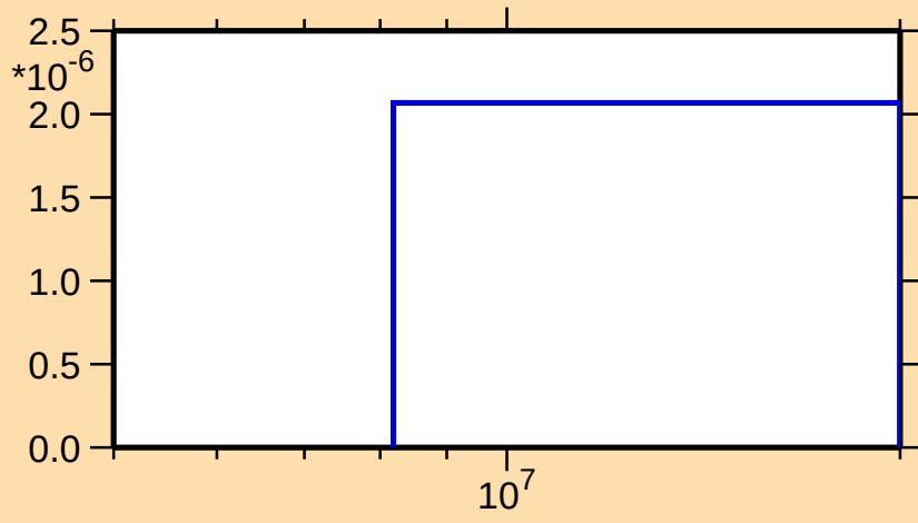
\sigma vs. E for ^{90}\text{Kr}(n,n\alpha)
