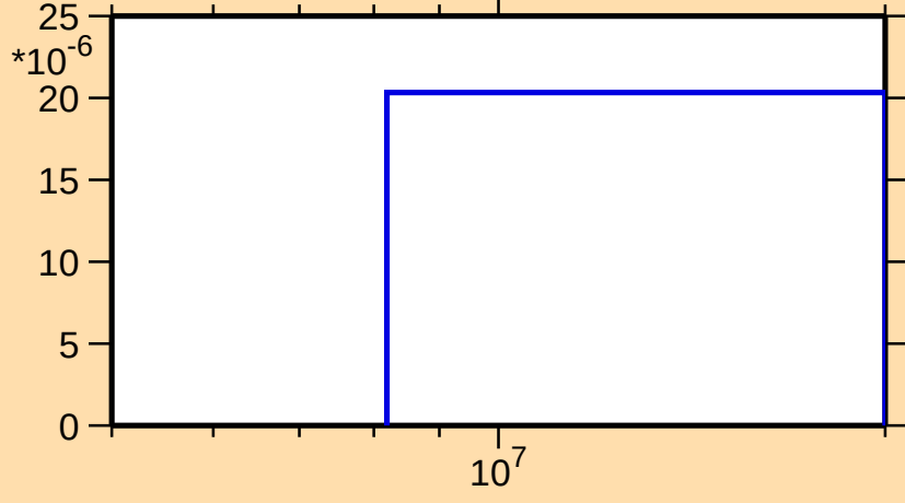
\sigma vs. E for ^{90}\text{Kr}(n,p)
