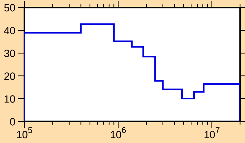
\Delta\sigma/\sigma vs. E for ^{90}\text{Kr}(n,\text{nonel.})
