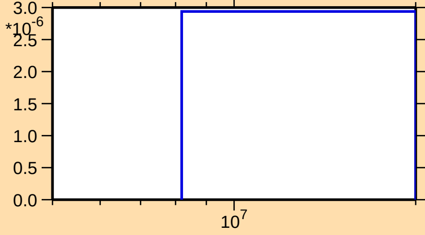
\sigma vs. E for ^{90}\text{Kr}(n,d)
