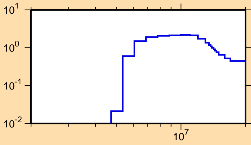
\sigma vs. E for ^{182}\text{Lu}(n,2n)
