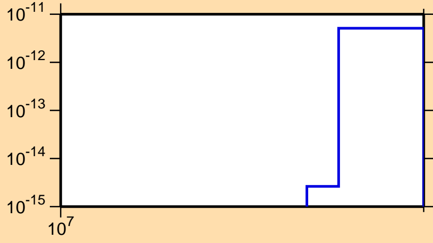
\sigma vs. E for ^{182}\text{Lu}(n,3n\alpha)
