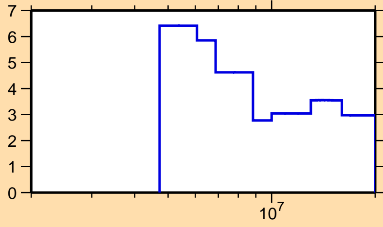
\Delta\sigma/\sigma vs. E for ^{182}\text{Lu}(n,\text{tot.})
