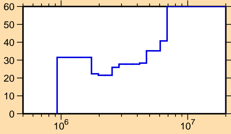
\Delta\sigma/\sigma vs. E for ^{253}\text{Md}(n,n\text{cont.})
