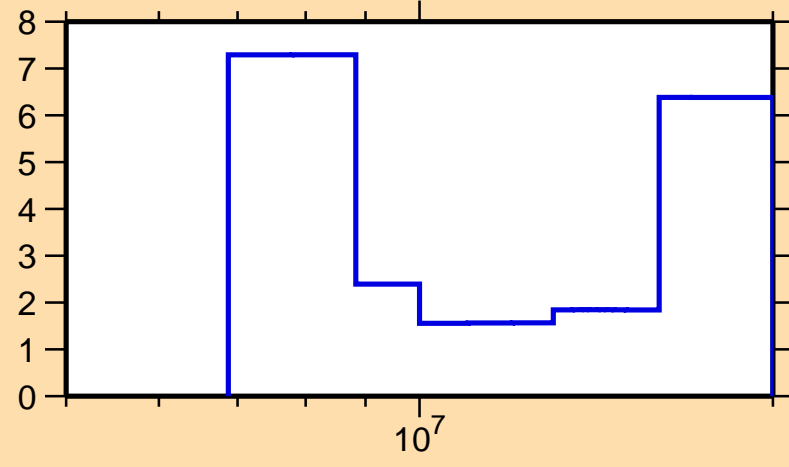
\Delta\sigma/\sigma vs. E for ^{253}\text{Md}(n,\text{el.})
