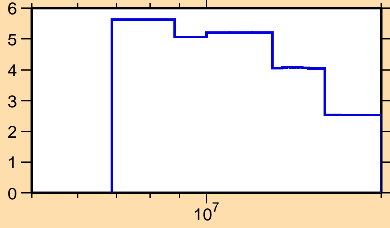
\Delta\sigma/\sigma vs. E for ^{253}\text{Md}(n,\text{tot.})
