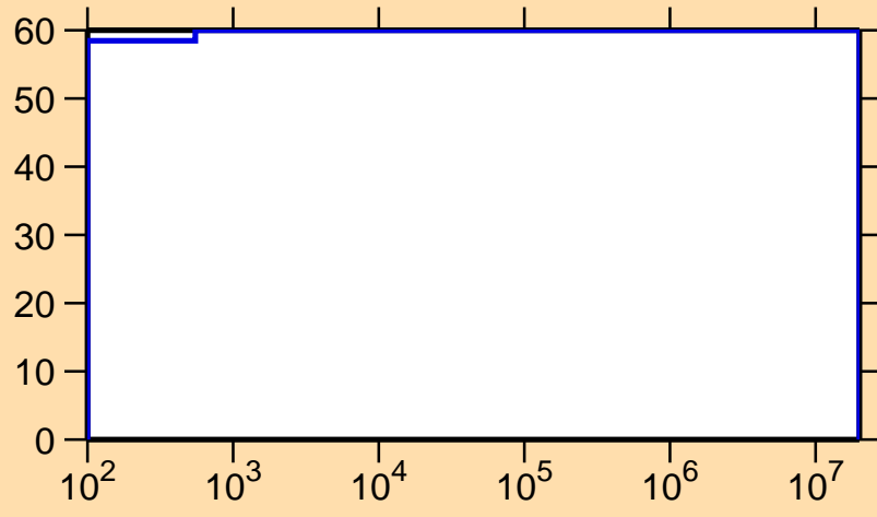
\Delta\sigma/\sigma vs. E for ^{258}\text{Md}(n,\gamma)
