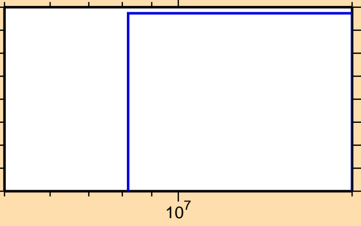
\sigma vs. E for ^{258}\text{Md}(\text{mt } 45)
