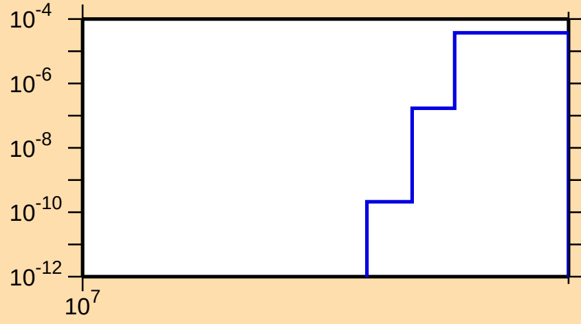
\sigma vs. E for ^{139}\text{Nd}(n,2np)
