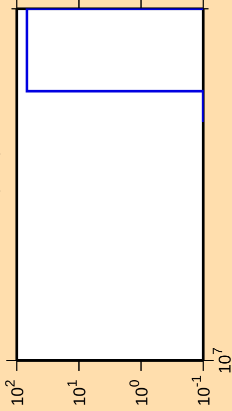
\Delta\sigma/\sigma vs. E for ^{139}\text{Nd}(n,\text{nt})
