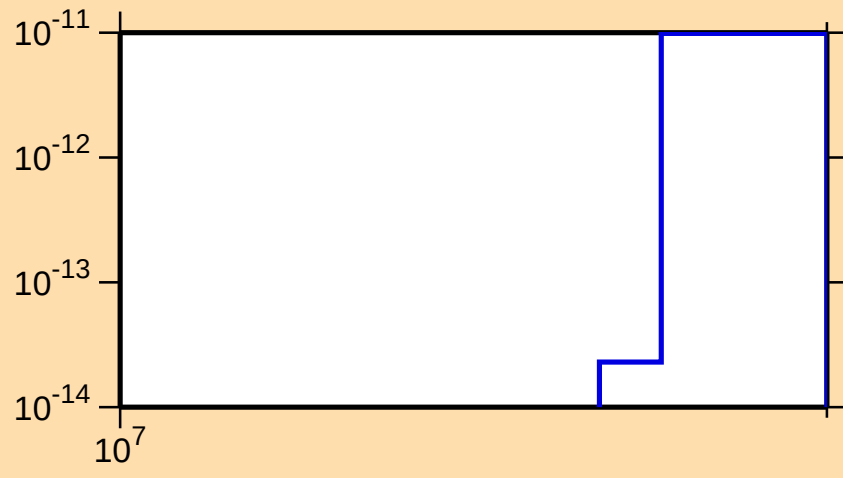
\sigma vs. E for ^{139}\text{Nd}(\text{mt } 34)
