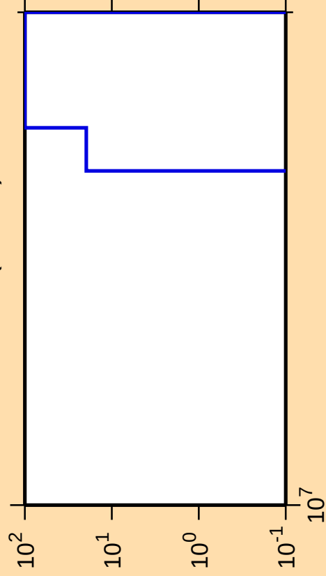
\Delta\sigma/\sigma vs. E for ^{139}\text{Nd}(\text{mt117})
