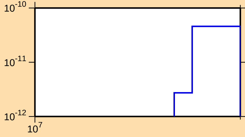
\sigma vs. E for ^{139}\text{Nd}(\text{mt117})
