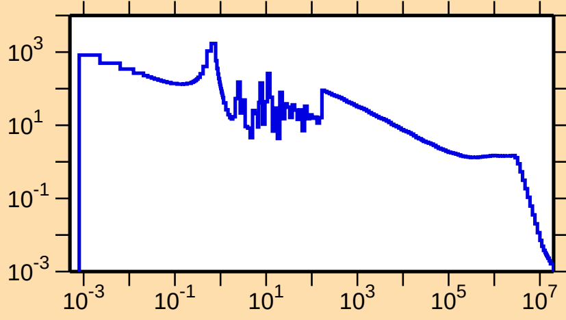
\sigma vs. E for ^{139}\text{Nd}(n,\gamma)
