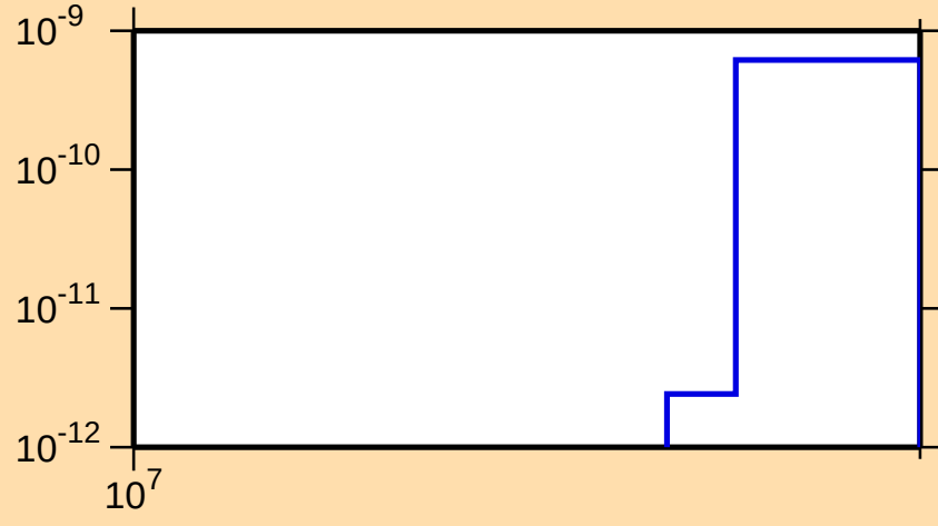
\sigma vs. E for ^{139}\text{Nd}(n,\text{pt})
