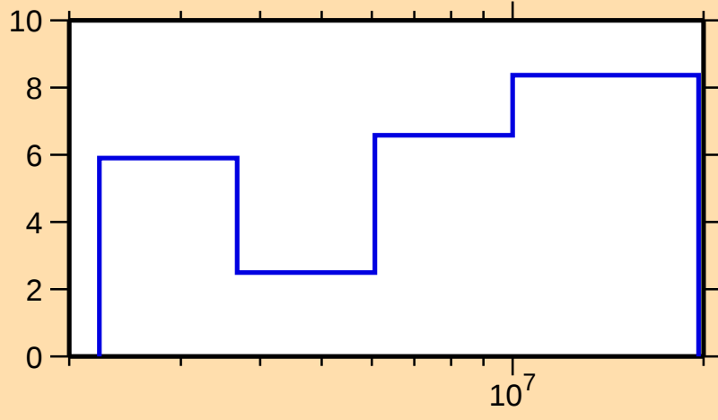
\Delta\sigma/\sigma vs. E for ^{65}\text{Ni}(n,\text{tot.})
