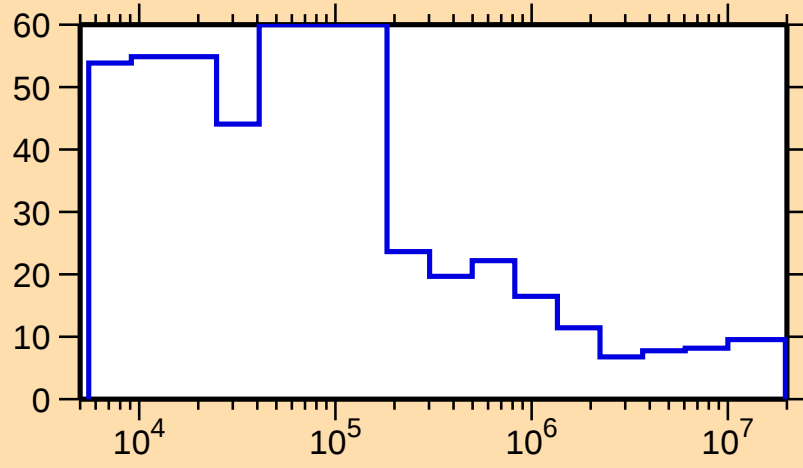
\Delta\sigma/\sigma vs. E for ^{65}\text{Ni}(n,\text{nonel.})
