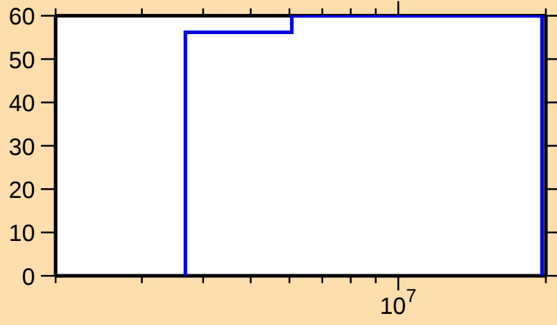
\Delta\sigma/\sigma vs. E for ^{65}\text{Ni}(n,\gamma)
