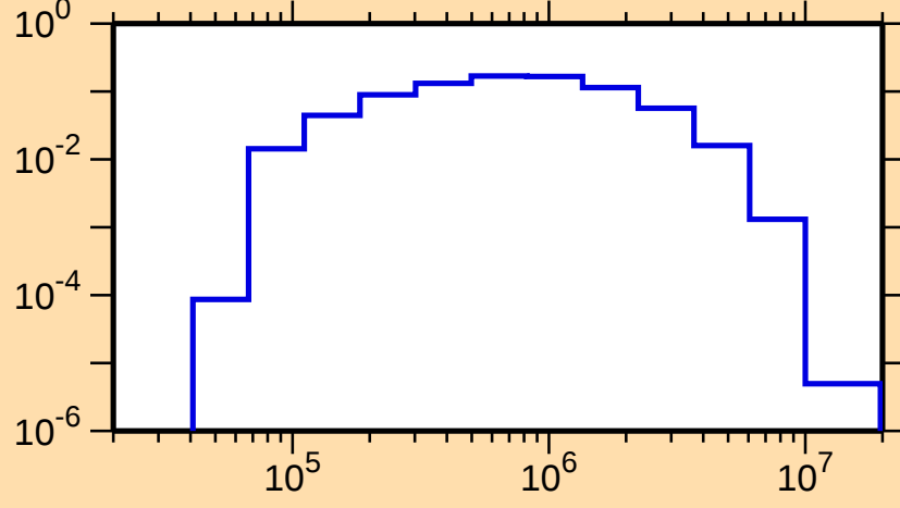
\sigma vs. E for ^{65}\text{Ni}(n,n_1)
