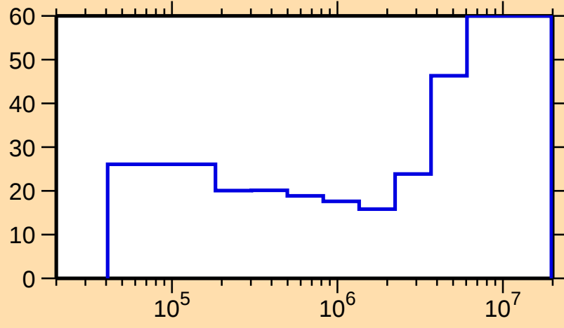
\Delta\sigma/\sigma vs. E for ^{65}\text{Ni}(n,n_1)
