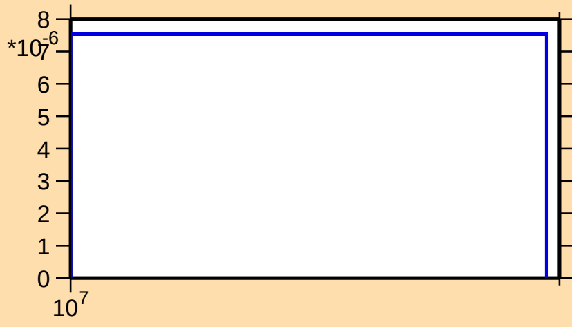
\sigma vs. E for ^{65}\text{Ni}(n,t)
