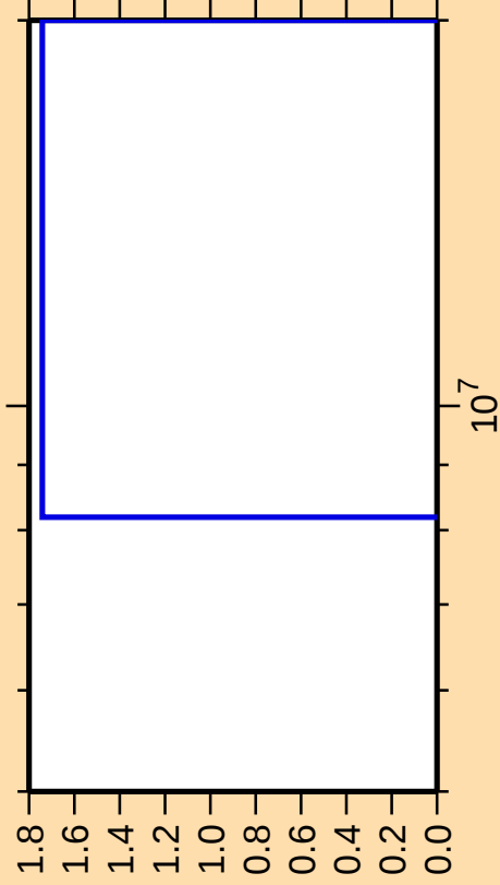
\Delta\sigma/\sigma vs. E for ^{236}\text{Np}(\text{mt117})
