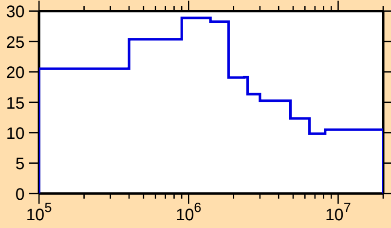
\Delta\sigma/\sigma vs. E for ^{236}\text{Np}(n,\text{tot.})
