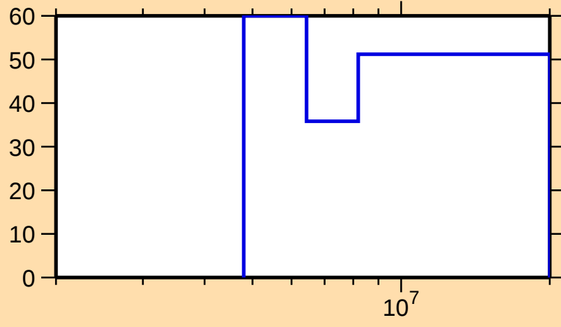
\Delta\sigma/\sigma vs. E for ^{236}\text{Np}(n,2n)
