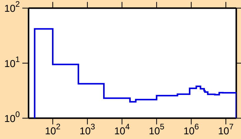
\sigma vs. E for ^{236}\text{Np}(n,\text{nonel.})
