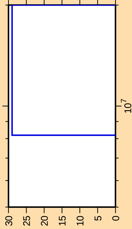
\Delta\sigma/\sigma vs. E for ^{236}\text{Np}(n,\text{nd})
