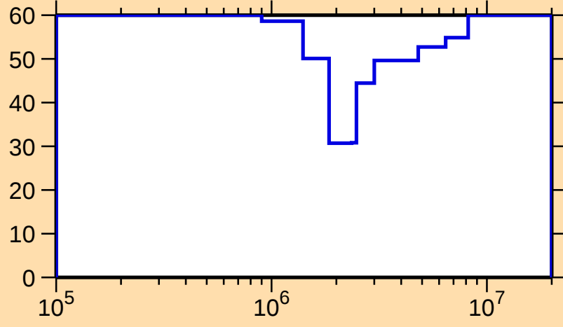
\Delta\sigma/\sigma vs. E for ^{236}\text{Np}(n,n_1)
