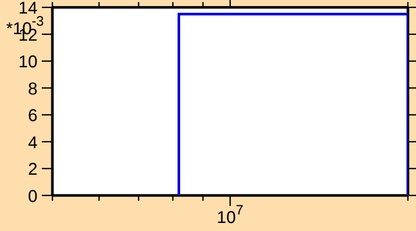
\sigma vs. E for ^{236}\text{Np}(n,3n)
