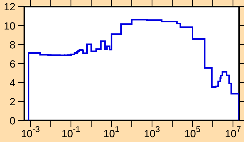
\sigma vs. E for ^{236}\text{Np}(n,\text{el.})
