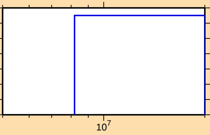
\sigma vs. E for ^{236}\text{Np}(n,2np)
