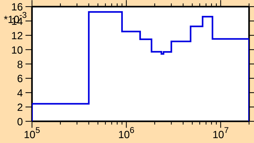
\sigma vs. E for ^{236}\text{Np}(n,n_2)
