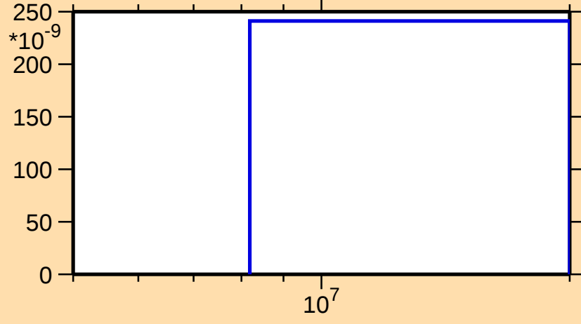
\sigma vs. E for ^{236}\text{Np}(n,\text{nd})
