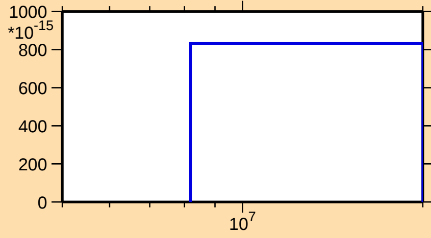
\sigma vs. E for ^{236}\text{Np}(\text{mt117})
