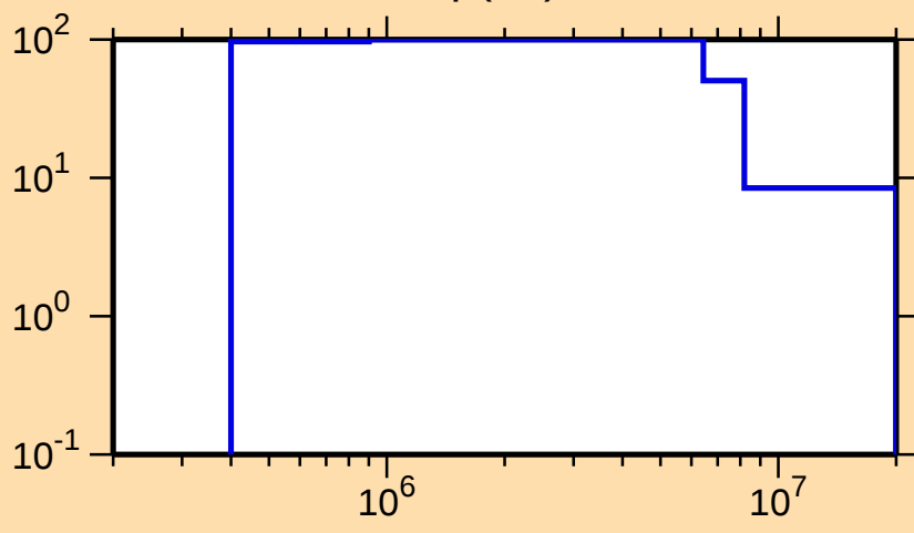
\Delta\sigma/\sigma vs. E for ^{236}\text{Np}(n,f)
