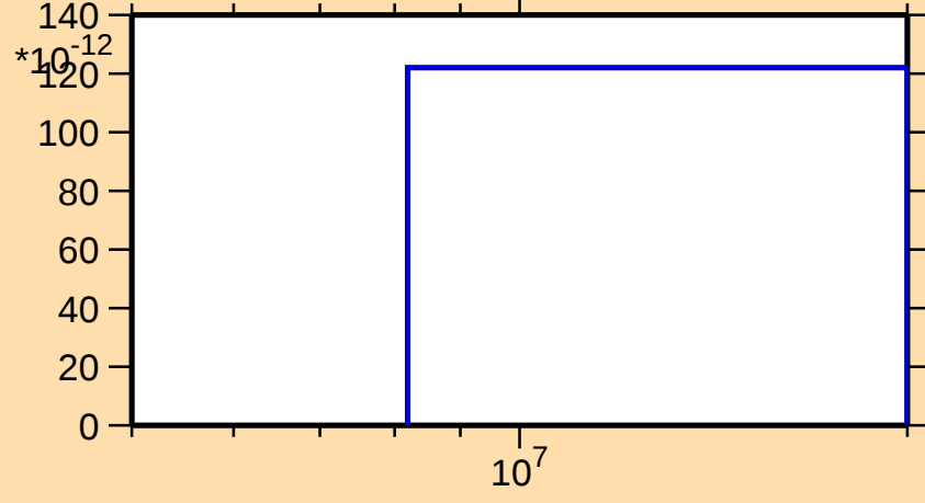
\sigma vs. E for ^{236}\text{Np}(n,p\alpha)
