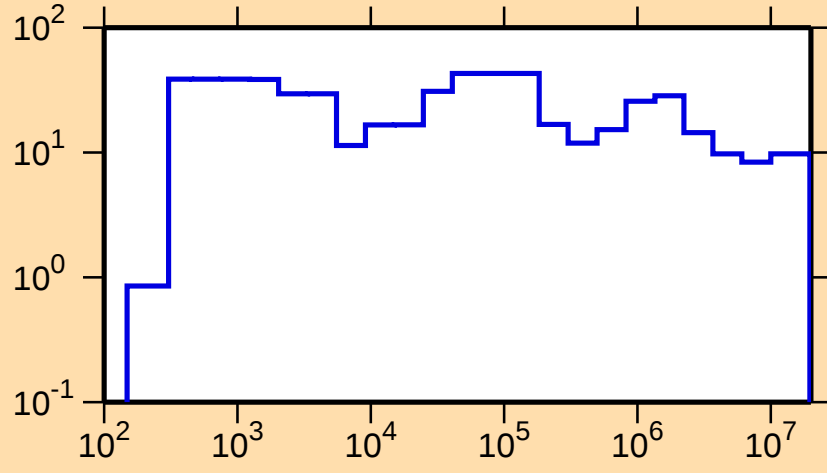
\Delta\sigma/\sigma vs. E for ^{176}\text{Os}(n,\text{nonel.})
