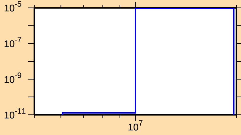
\sigma vs. E for ^{176}\text{Os}(n,2n\alpha)
