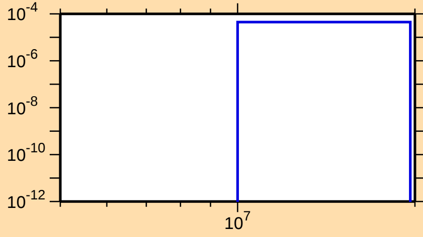
\sigma vs. E for ^{176}\text{Os}(n,t)
