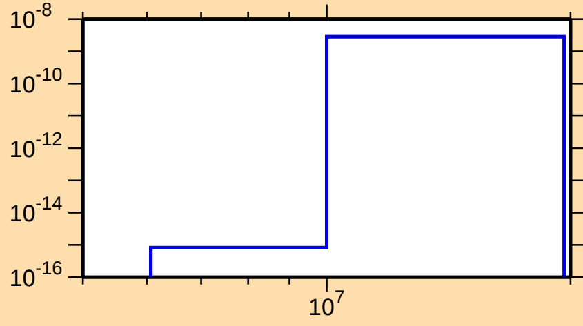
\sigma vs. E for ^{176}\text{Os}(\text{mt117})
