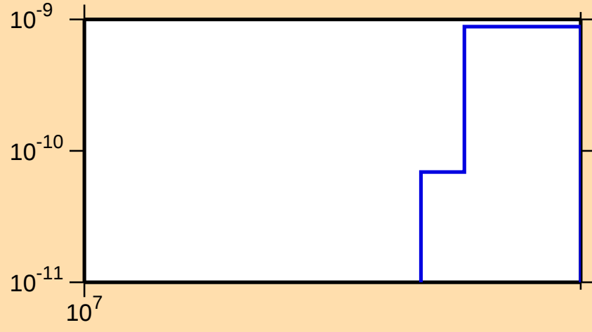
\sigma vs. E for ^{230}\text{Pa}(n,\text{He}3)
