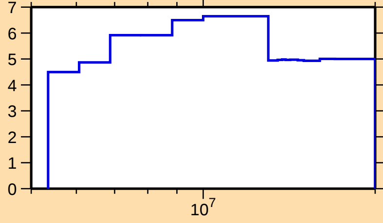
\Delta\sigma/\sigma vs. E for ^{230}\text{Pa}(n,\text{nonel.})
