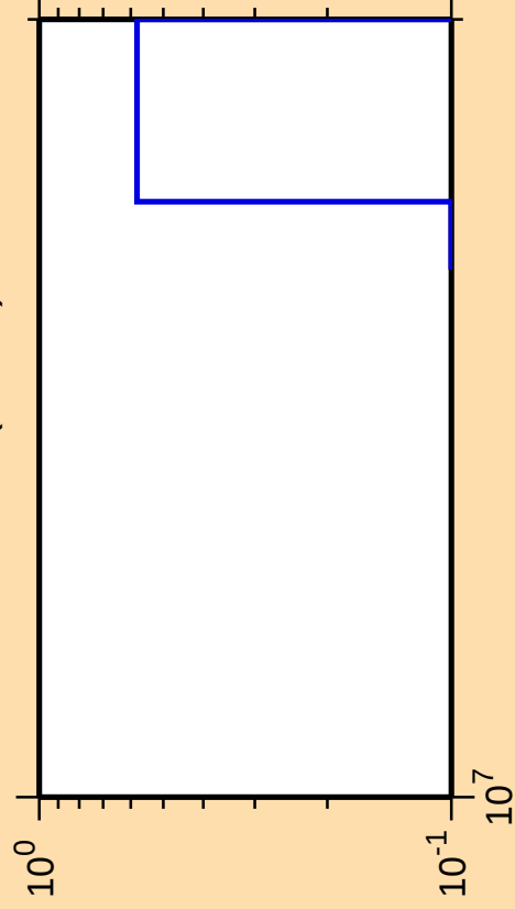
\Delta\sigma/\sigma vs. E for ^{230}\text{Pa} (mt 11)
