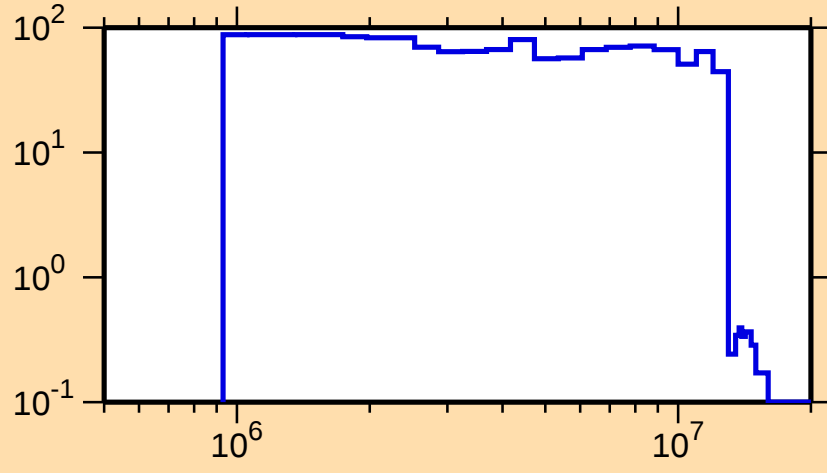
\Delta\sigma/\sigma vs. E for ^{230}\text{Pa}(n,n_1)
