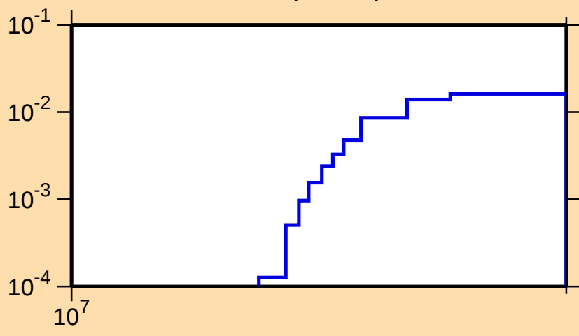
\sigma vs. E for ^{230}\text{Pa}(n,3n\alpha)
