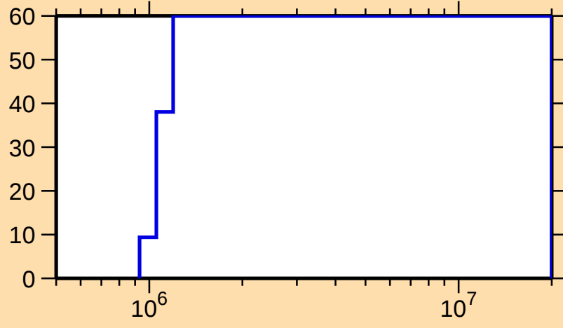
\Delta\sigma/\sigma vs. E for ^{230}\text{Pa}(n,p)
