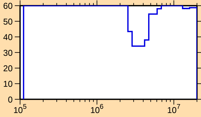
\Delta\sigma/\sigma vs. E for ^{230}\text{Pa}(n,\text{inel.})
