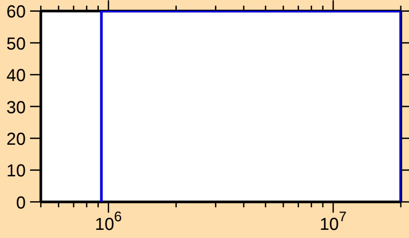
\Delta\sigma/\sigma vs. E for ^{230}\text{Pa}(n,\gamma)
