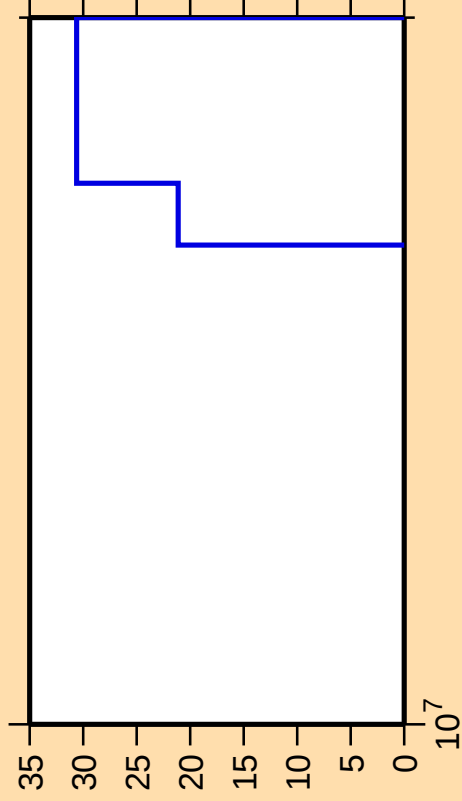
\Delta\sigma/\sigma vs. E for ^{230}\text{Pa}(n,\text{He}3)
