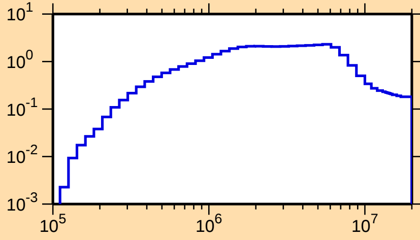
\sigma vs. E for ^{230}\text{Pa}(n,n\text{cont.})
