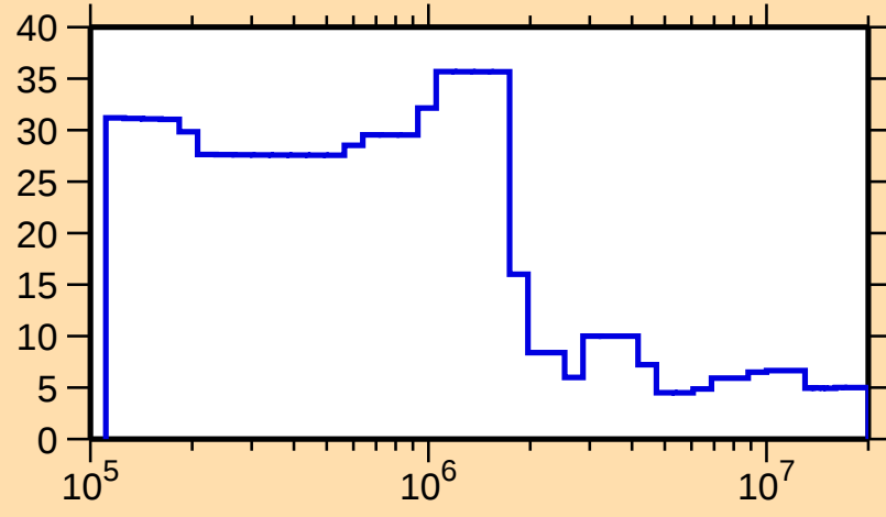
\Delta\sigma/\sigma vs. E for ^{230}\text{Pa}(n,\text{nonel.})
