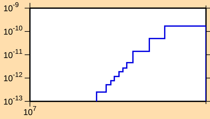
\sigma vs. E for ^{230}\text{Pa}(\text{mt117})
