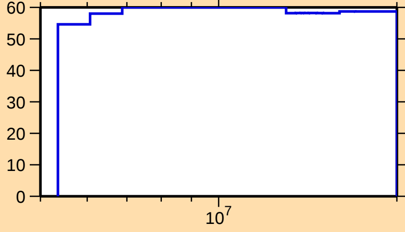
\Delta\sigma/\sigma vs. E for ^{230}\text{Pa}(n,\text{inel.})
