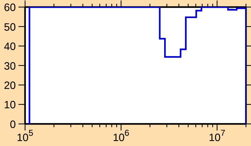
\Delta\sigma/\sigma vs. E for ^{230}\text{Pa}(n,n\text{cont.})
