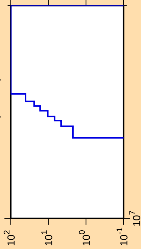
\Delta\sigma/\sigma vs. E for ^{230}\text{Pa}(\text{mt117})
