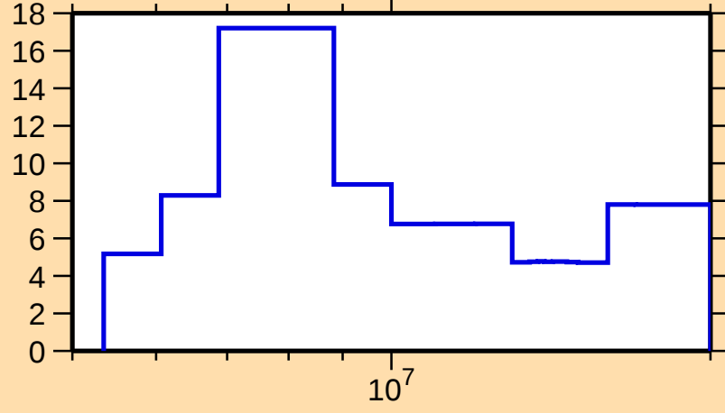
\Delta\sigma/\sigma vs. E for ^{230}\text{Pa}(n,\text{tot.})
