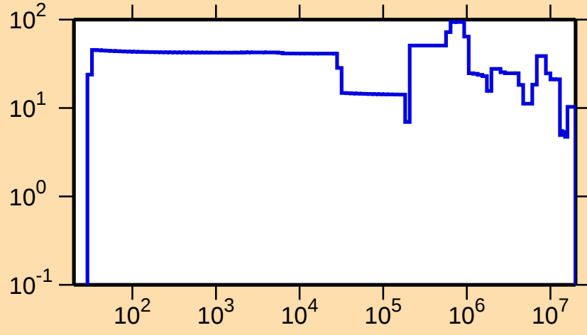
\Delta\sigma/\sigma vs. E for ^{230}\text{Pa}(n,\text{el.})
