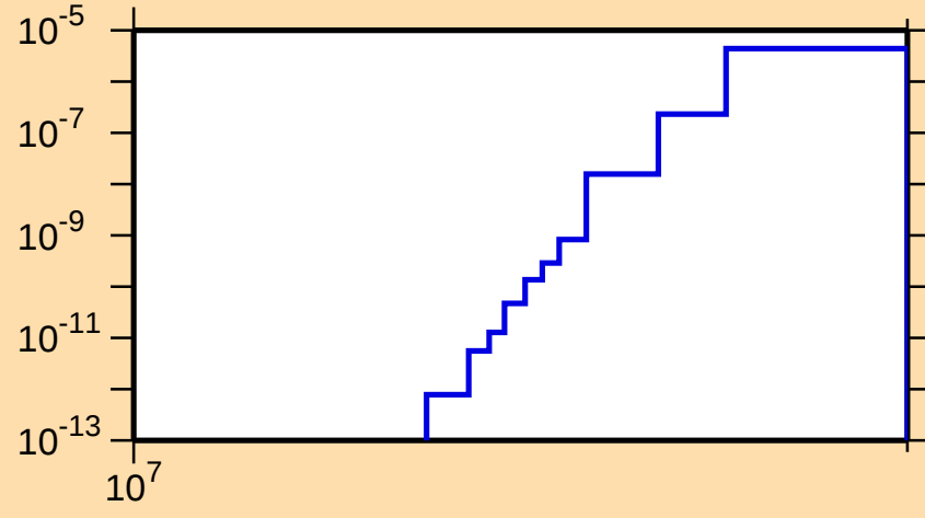
\sigma vs. E for ^{230}\text{Pa}(n,nt)
