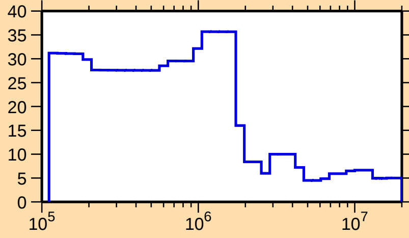
\Delta\sigma/\sigma vs. E for ^{230}\text{Pa}(n,\text{nonel.})
