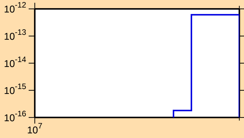
\sigma vs. E for ^{230}\text{Pa} (mt 11)
