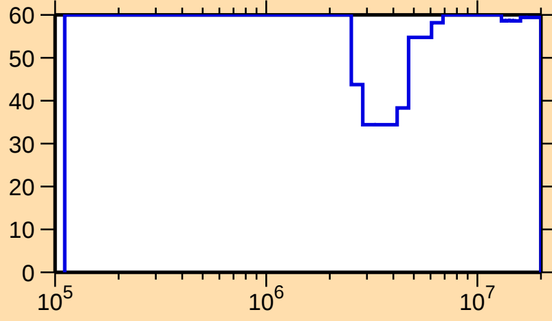
\Delta\sigma/\sigma vs. E for ^{230}\text{Pa}(n,n\text{cont.})
