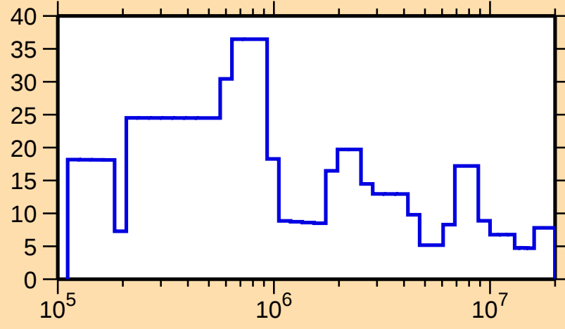
\Delta\sigma/\sigma vs. E for ^{230}\text{Pa}(n,\text{tot.})
