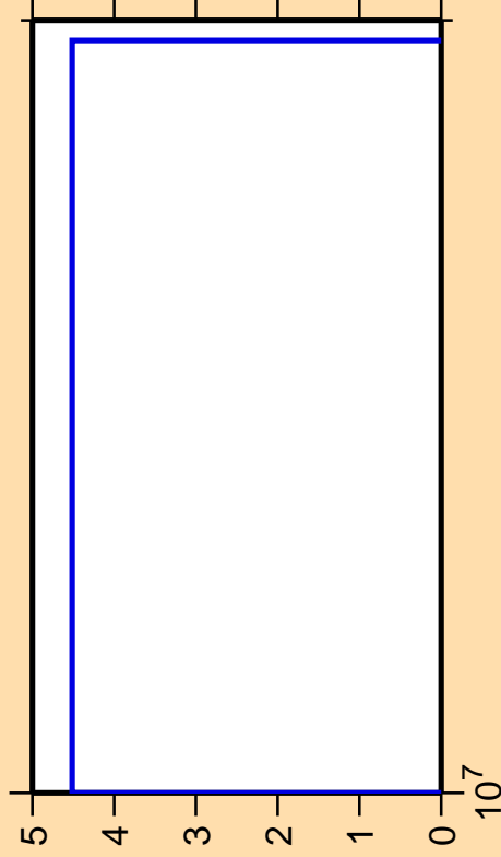
\Delta\sigma/\sigma vs. E for ^{197}\text{Pb} (mt 45)
