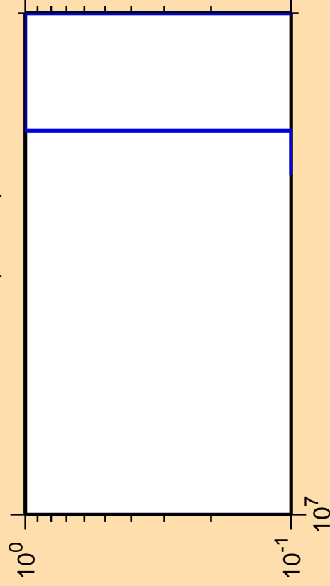
\Delta\sigma/\sigma vs. E for ^{201}\text{Pb}(\text{mt } 45)
