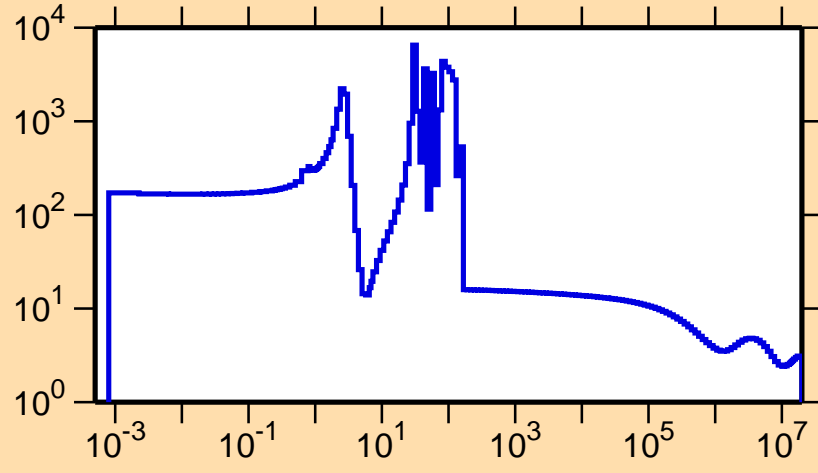
\sigma vs. E for ^{201}\text{Pb}(n,\text{el.})
