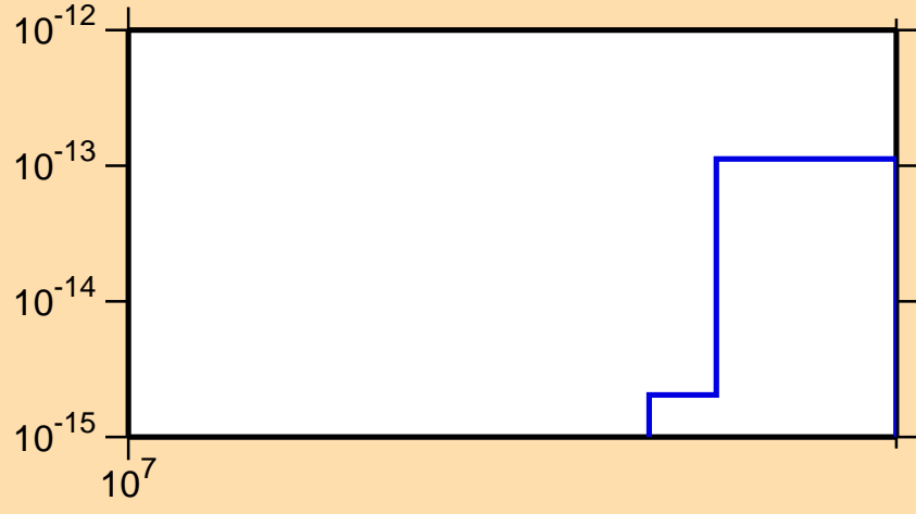
\sigma vs. E for ^{201}\text{Pb}(\text{mt } 45)
