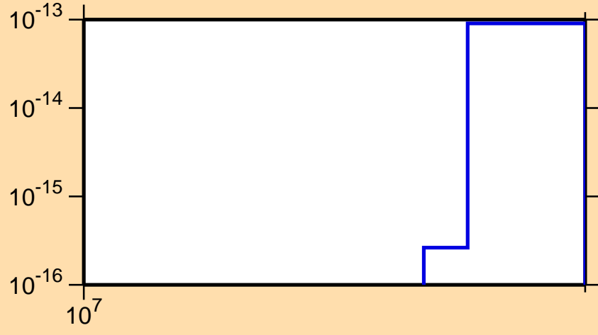
\sigma vs. E for ^{201}\text{Pb} (mt 34)
