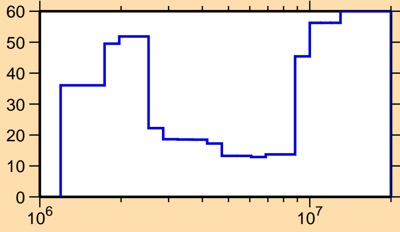
\Delta\sigma/\sigma vs. E for ^{201}\text{Pb}(n,n\text{cont.})
