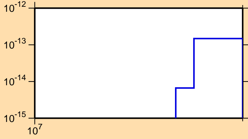
\sigma vs. E for ^{201}\text{Pb}(\text{mt117})
