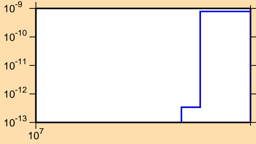
\sigma vs. E for ^{201}\text{Pb}(n,nt)
