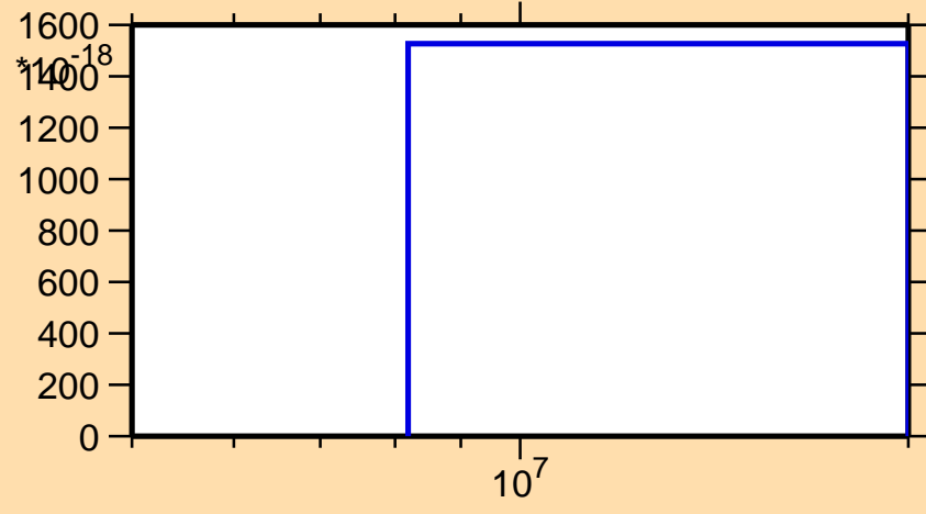
\sigma vs. E for ^{201}\text{Pb}(\text{mt117})
