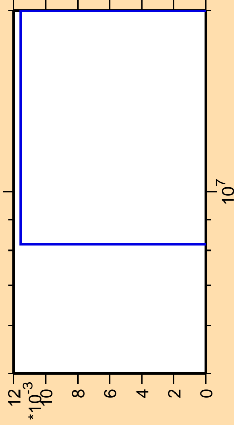
\Delta\sigma/\sigma vs. E for ^{201}\text{Pb}(\text{mt117})
