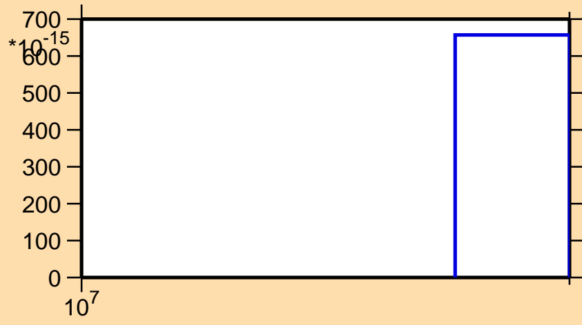
\sigma vs. E for ^{204}\text{Pb}(n,3n\alpha)
