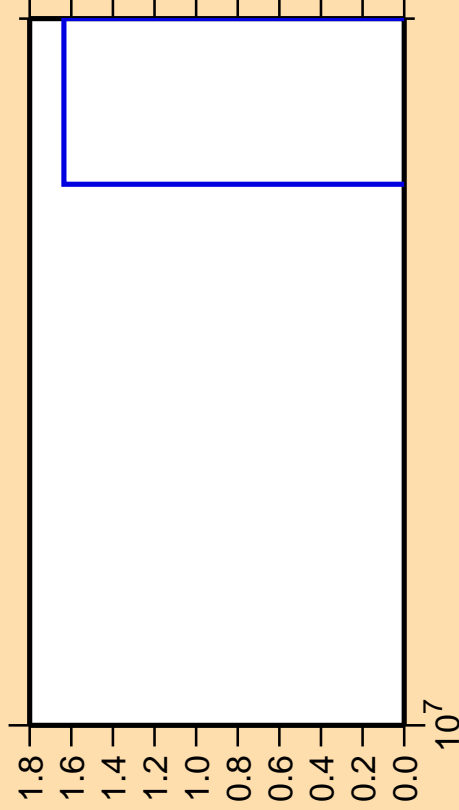
\Delta\sigma/\sigma vs. E for ^{204}\text{Pb}(n,3n\alpha)
