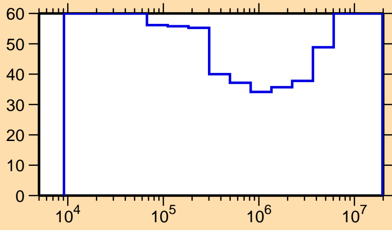
\Delta\sigma/\sigma vs. E for ^{204}\text{Pb}(n,\gamma)
