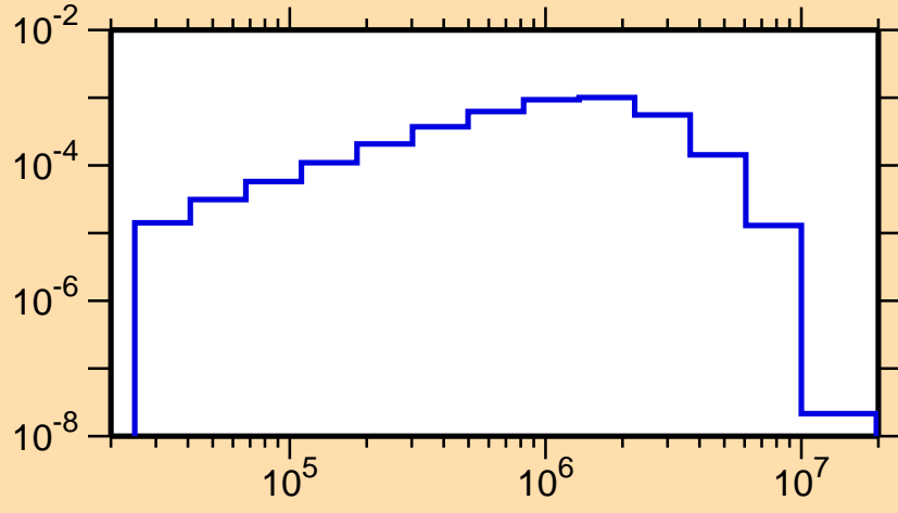
\sigma vs. E for ^{204}\text{Pb}(n,n_2)
