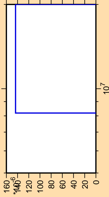
\Delta\sigma/\sigma vs. E for ^{204}\text{Pb}(\text{mt } 34)
