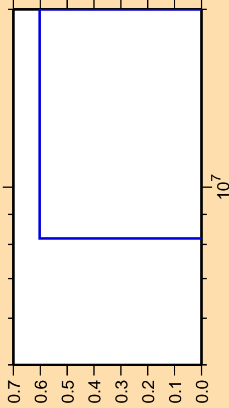
\Delta\sigma/\sigma vs. E for ^{204}\text{Pb}(\text{mt } 45)
