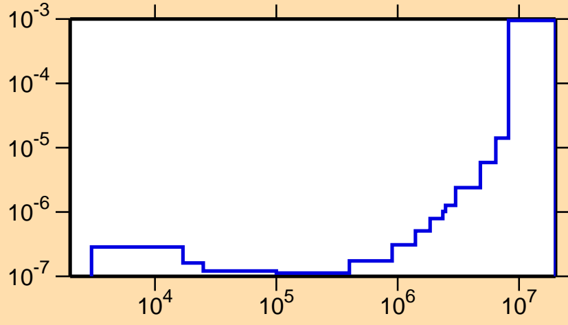
\sigma vs. E for ^{204}\text{Pb}(n,\alpha)
