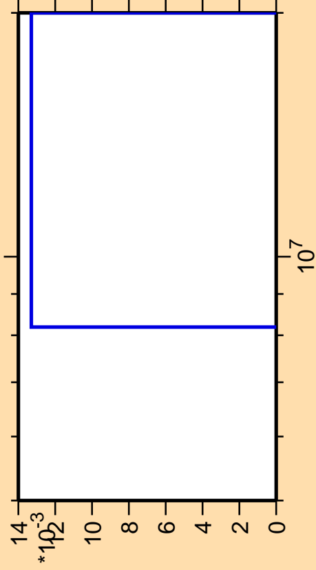
\Delta\sigma/\sigma vs. E for ^{204}\text{Pb}(n,3n\alpha)
