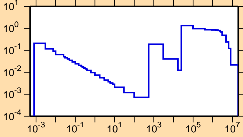
\sigma vs. E for ^{204}\text{Pb}(n,\gamma)
