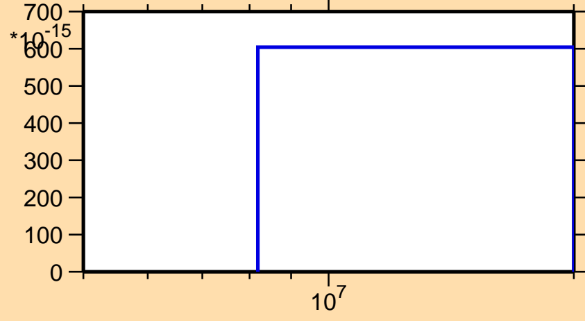
\sigma vs. E for ^{204}\text{Pb}(\text{mt } 45)
