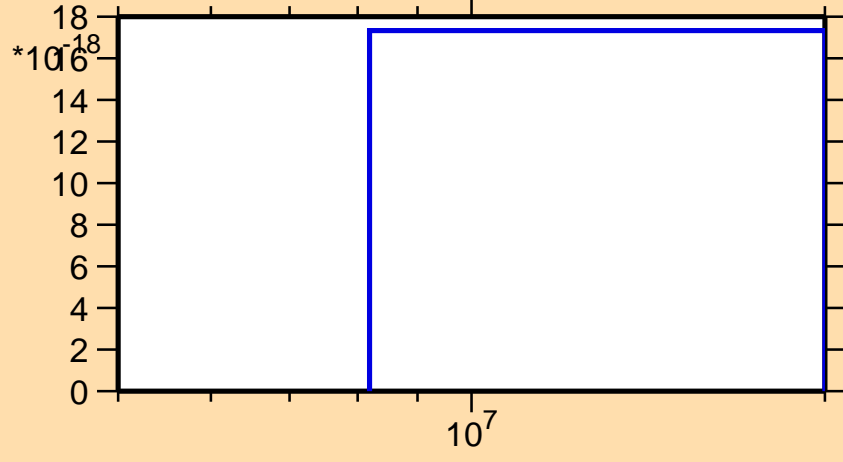
\sigma vs. E for ^{204}\text{Pb}(\text{mt } 34)
