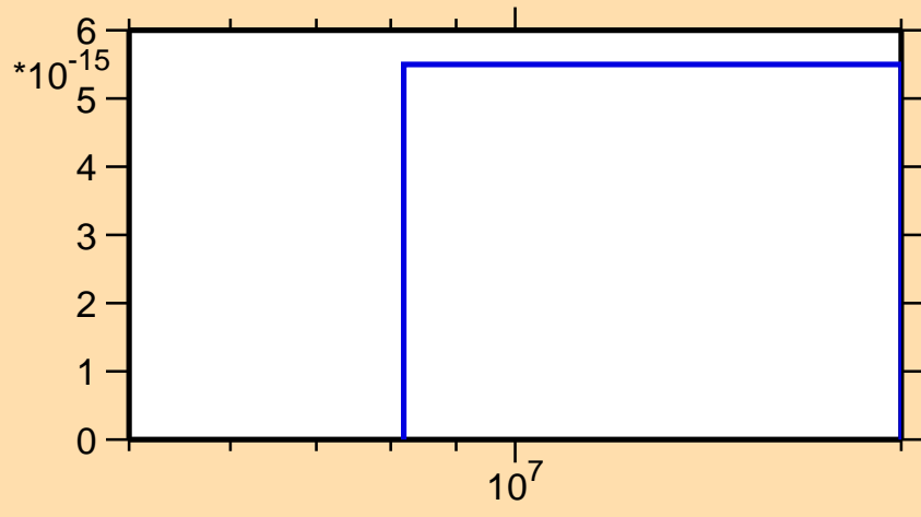
\sigma vs. E for ^{204}\text{Pb}(n,3n\alpha)
