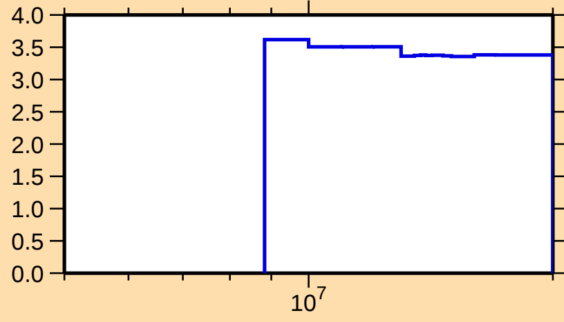
\Delta\sigma/\sigma vs. E for ^{106}\text{Pd}(n,\text{nonel.})
