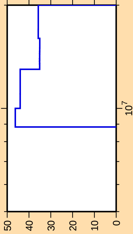
\Delta\sigma/\sigma vs. E for ^{106}\text{Pd}(n,\alpha)
