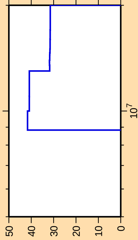
\Delta\sigma/\sigma vs. E for ^{106}\text{Pd}(n,p)
