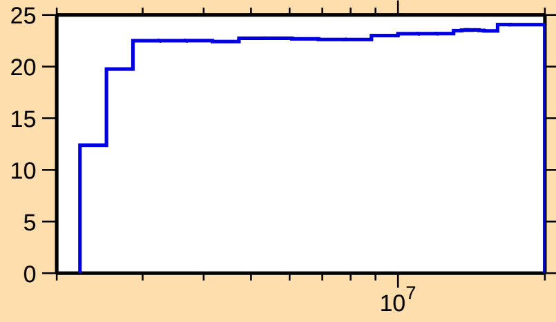
\Delta\sigma/\sigma vs. E for ^{106}\text{Pd}(n,n_1)
