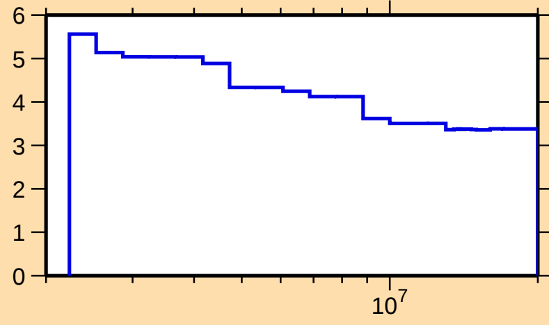
\Delta\sigma/\sigma vs. E for ^{106}\text{Pd}(n,\text{nonel.})
