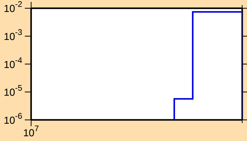
\sigma vs. E for ^{106}\text{Pd}(n,3n)
