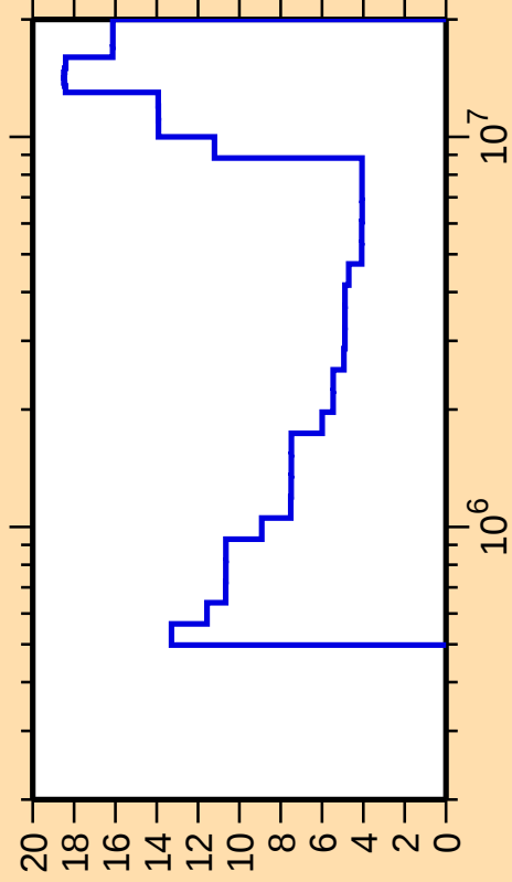
\Delta\sigma/\sigma vs. E for ^{106}\text{Pd}(n,\text{inel.})
