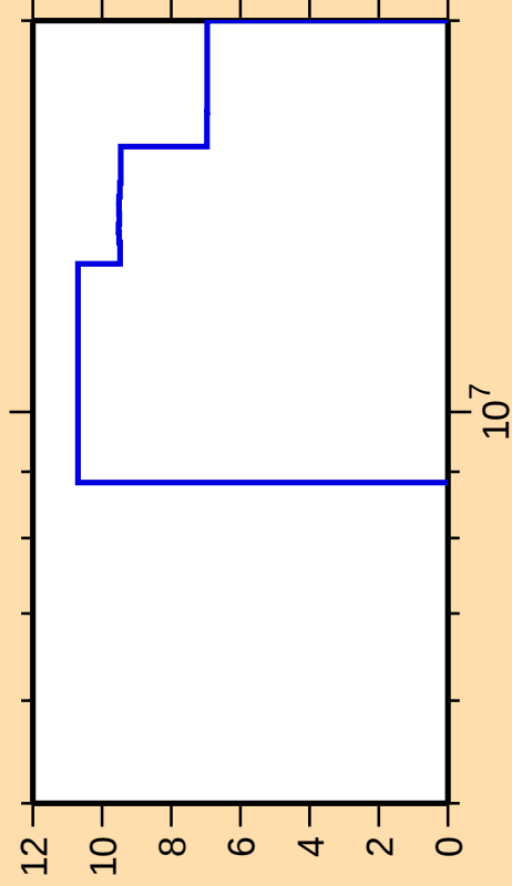
\Delta\sigma/\sigma vs. E for ^{106}\text{Pd}(n,2n)
