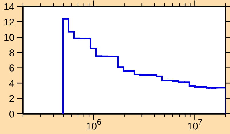
\Delta\sigma/\sigma vs. E for ^{106}\text{Pd}(n,\text{nonel.})
