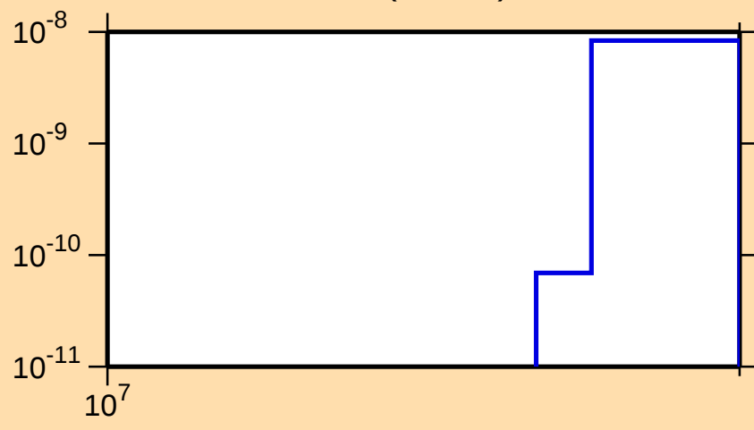
\sigma vs. E for ^{106}\text{Pd}(n,\text{He3})
