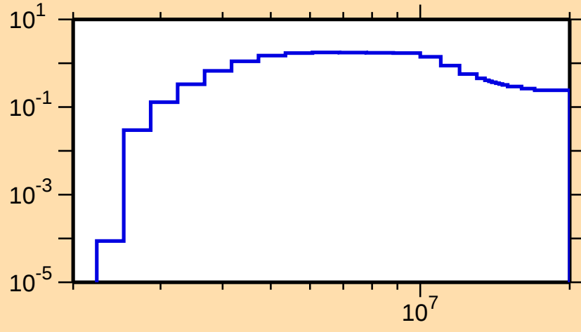
\sigma vs. E for ^{106}\text{Pd}(n,n\text{cont.})
