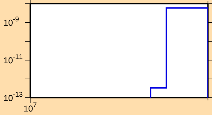
\sigma vs. E for ^{106}\text{Pd}(n,\text{nd})
