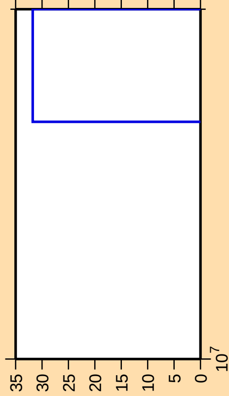
\Delta\sigma/\sigma vs. E for ^{106}\text{Pd}(n,3n)
