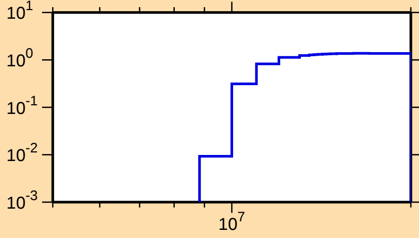
\sigma vs. E for ^{106}\text{Pd}(n,2n)
