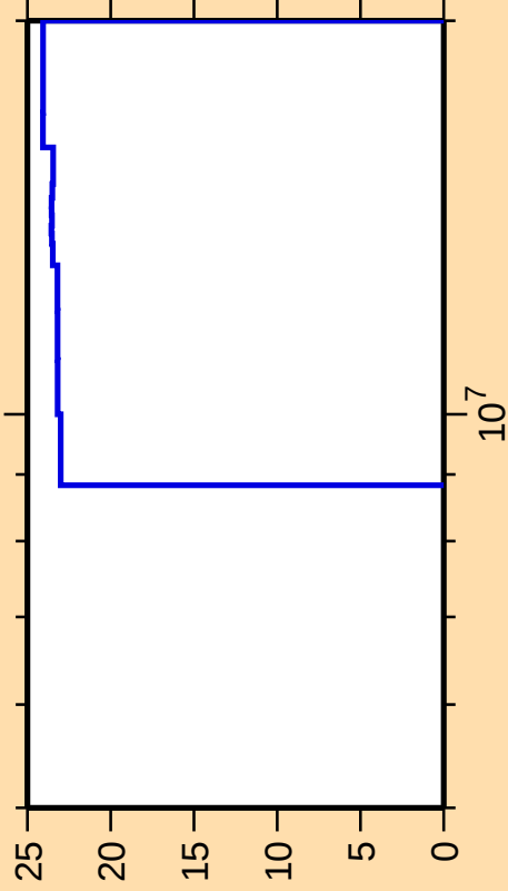
\Delta\sigma/\sigma vs. E for ^{106}\text{Pd}(n,n_1)
