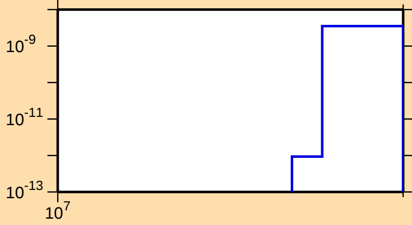
\sigma vs. E for ^{106}\text{Pd}(n,2n\alpha)
