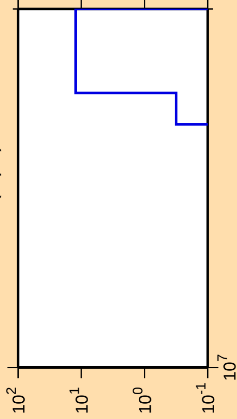
\Delta\sigma/\sigma vs. E for ^{106}\text{Pd}(n,p\alpha)
