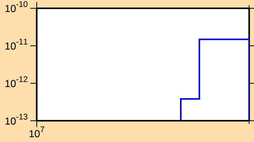
\sigma vs. E for ^{106}\text{Pd}(n,p\alpha)
