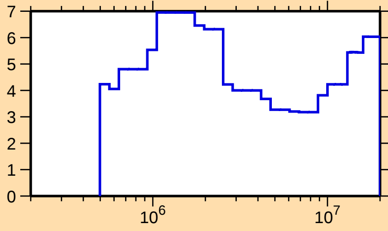
\Delta\sigma/\sigma vs. E for ^{106}\text{Pd}(n,\text{tot.})
