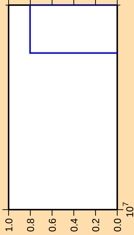
\Delta\sigma/\sigma vs. E for ^{106}\text{Pd}(n,2np)
