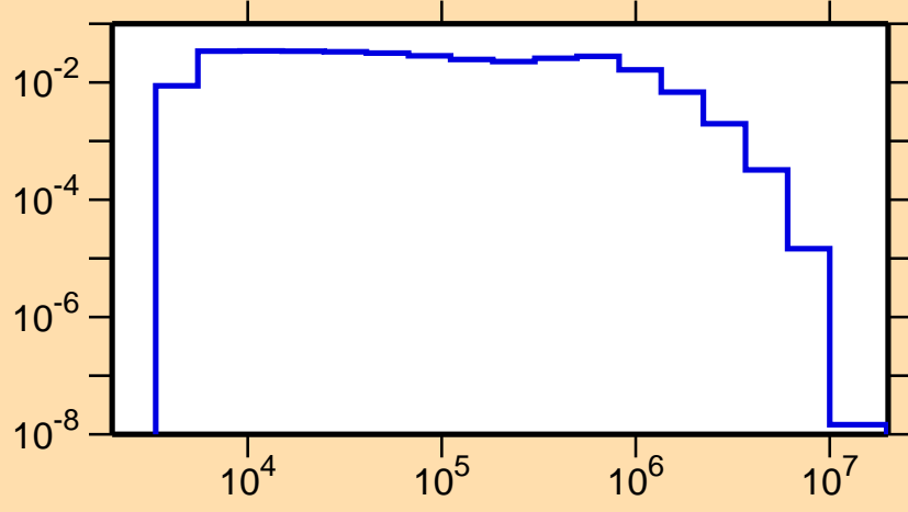
\sigma vs. E for ^{109}\text{Pd}(n,n_1)
