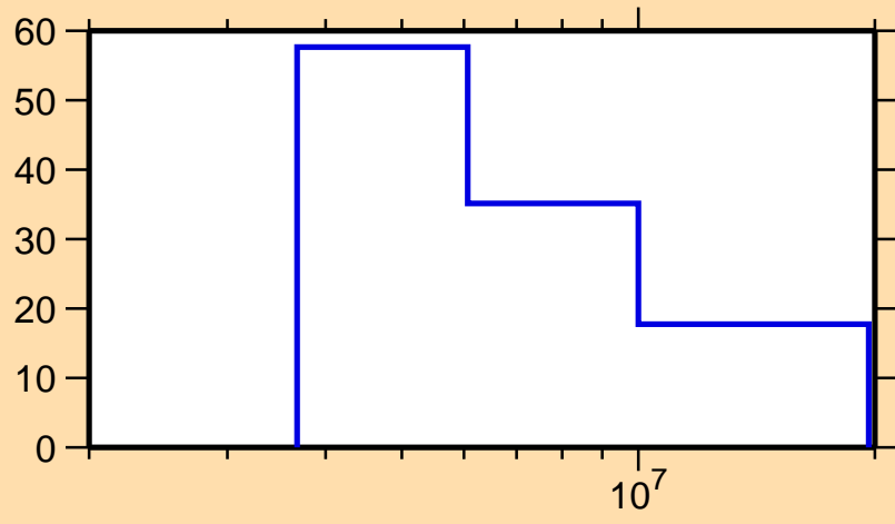
\Delta\sigma/\sigma vs. E for ^{109}\text{Pd}(n,2n)
