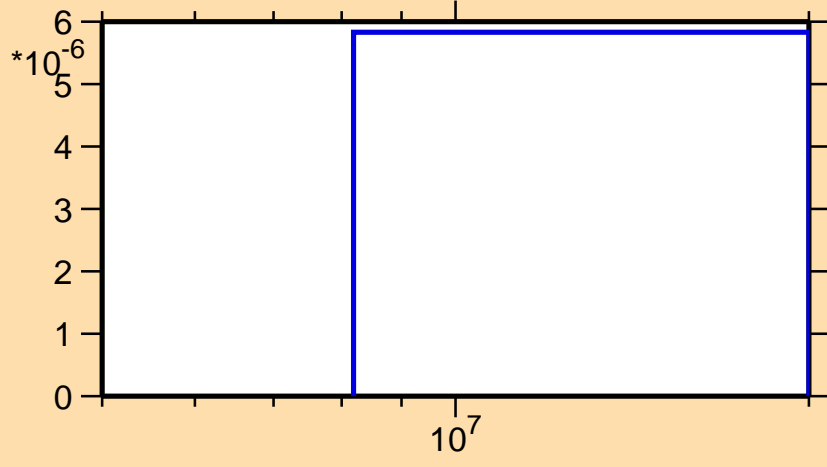
\sigma vs. E for ^{159}\text{Pm}(n,t)
