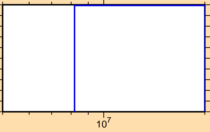
\sigma vs. E for ^{159}\text{Pm}(n,nd)
