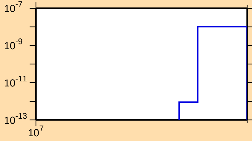
\sigma vs. E for ^{131}\text{Pr}(n,nt)
