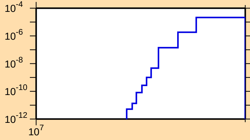
\sigma vs. E for ^{131}\text{Pr}(n,\text{nd})
