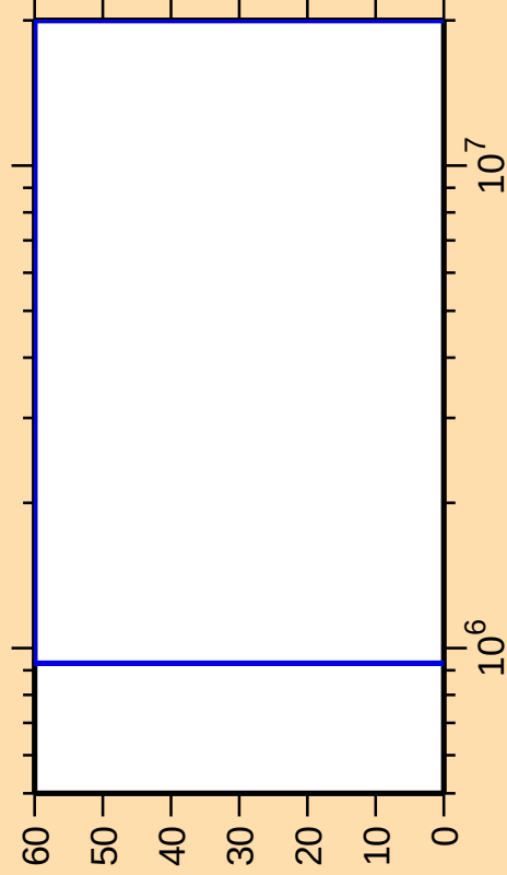
\Delta\sigma/\sigma vs. E for ^{131}\text{Pr}(n,p\alpha)
