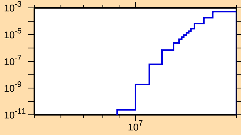
\sigma vs. E for ^{131}\text{Pr}(\text{mt } 45)
