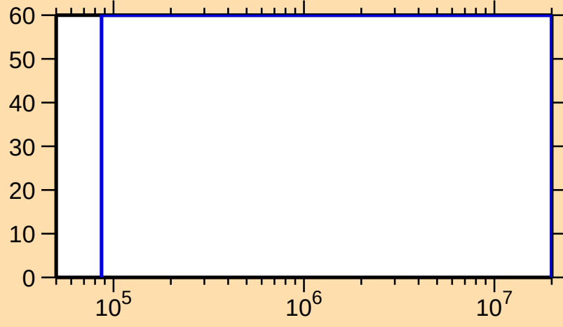
\Delta\sigma/\sigma vs. E for ^{131}\text{Pr}(n,n_1)
