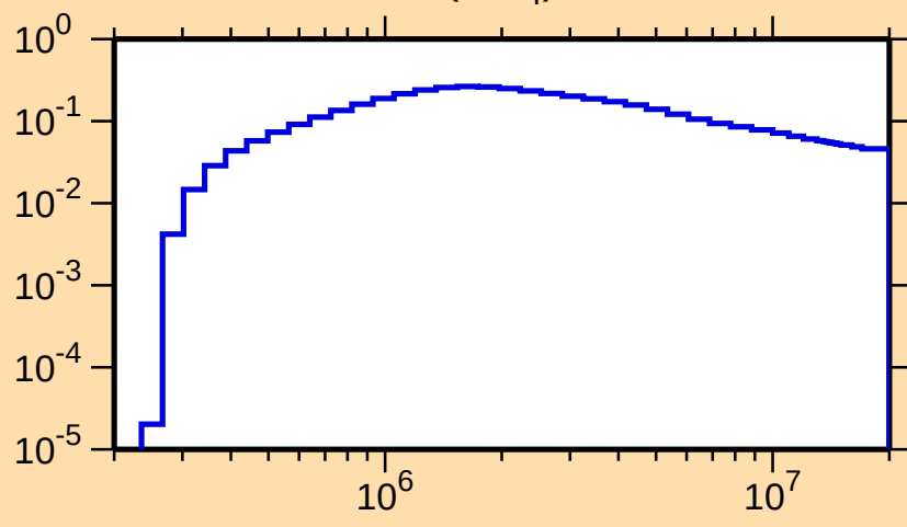
\sigma vs. E for ^{131}\text{Pr}(n,n_4)
