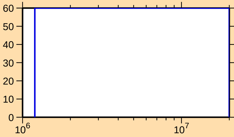
\Delta\sigma/\sigma vs. E for ^{131}\text{Pr}(n,\text{ncont.})
