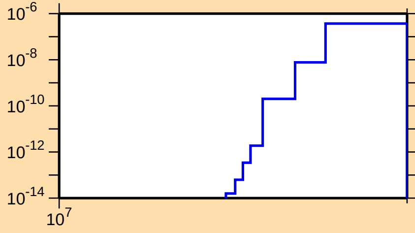
\sigma vs. E for ^{131}\text{Pr}(n,2n\alpha)
