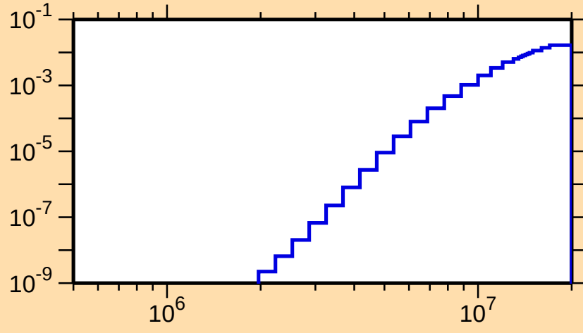
\sigma vs. E for ^{131}\text{Pr}(n,p\alpha)
