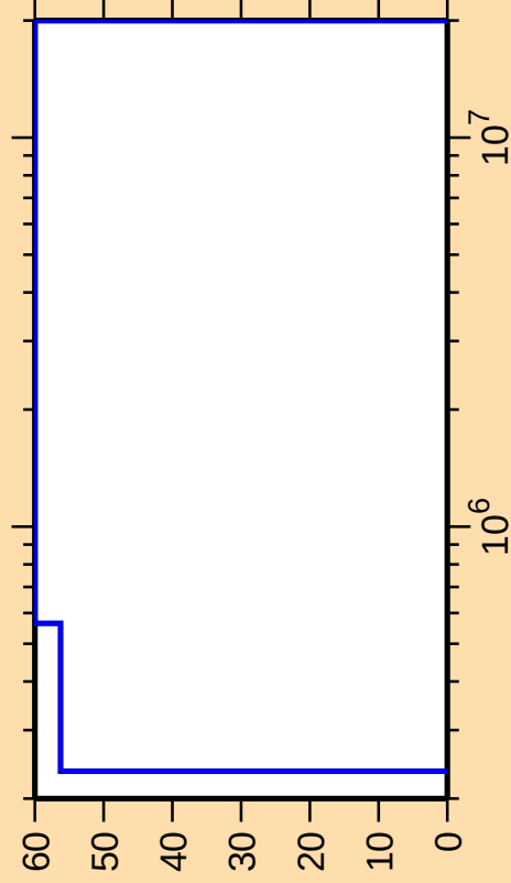
\Delta\sigma/\sigma vs. E for ^{131}\text{Pr}(n,n_4)
