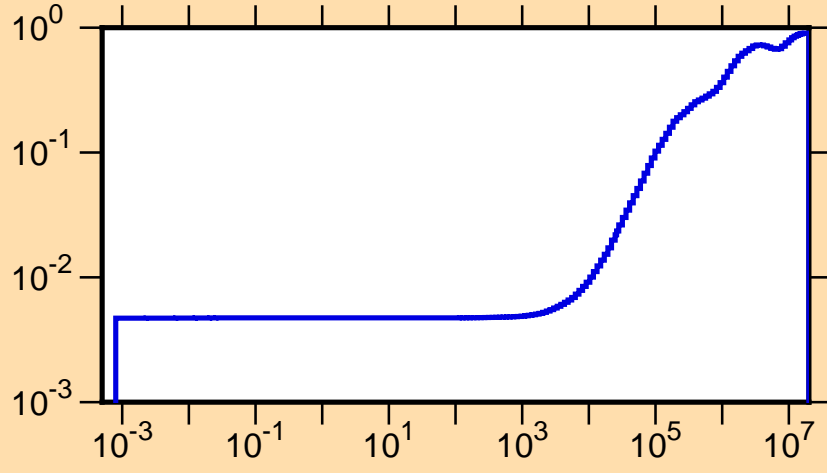
\mu vs. E for ^{143}\text{Pr}(\text{mt251})
