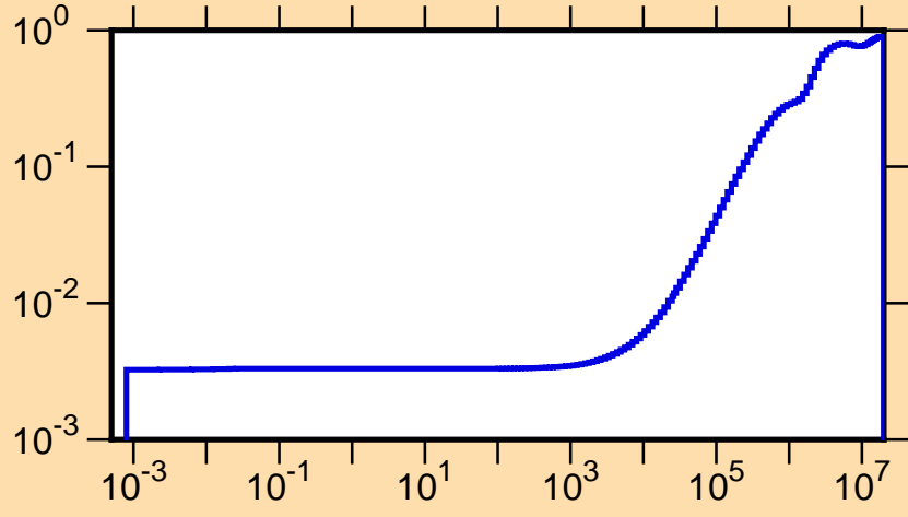
\mu vs. E for ^{207}\text{Ra}(\text{mt251})
