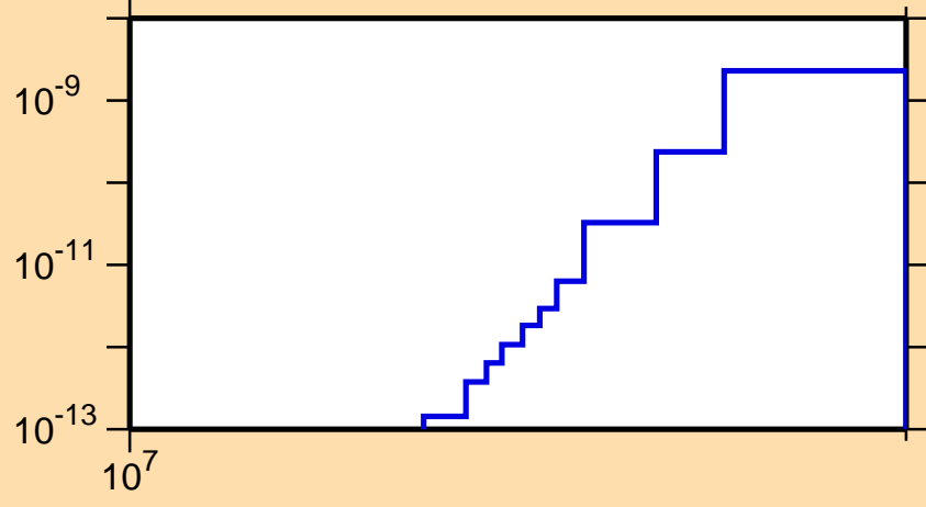
\sigma vs. E for ^{207}\text{Ra}(\text{mt } 34)
