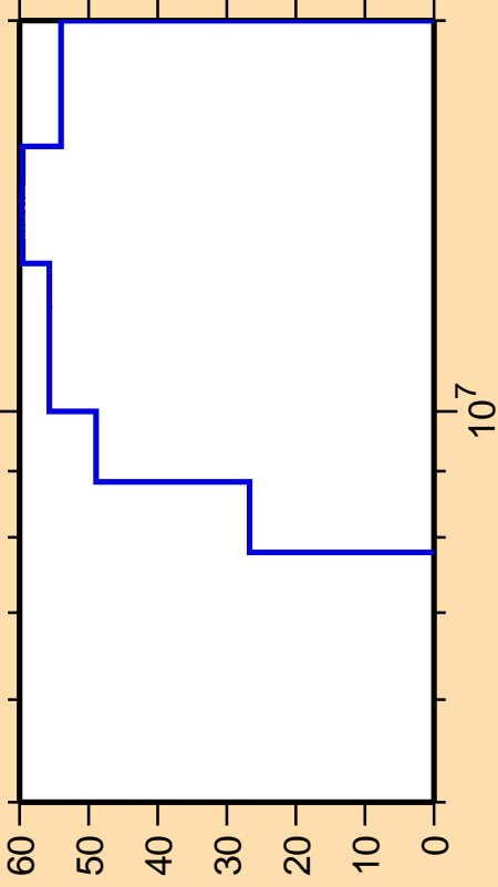
\Delta\sigma/\sigma vs. E for ^{207}\text{Ra}(n,n\text{cont.})
