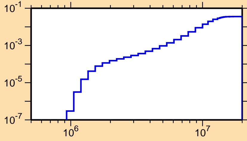
\sigma vs. E for ^{207}\text{Ra}(n,n\alpha)
