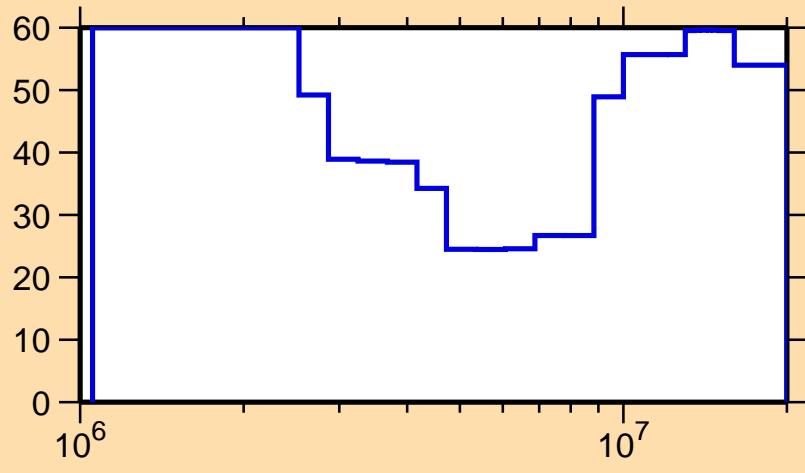
\Delta\sigma/\sigma vs. E for ^{207}\text{Ra}(n,n\text{cont.})
