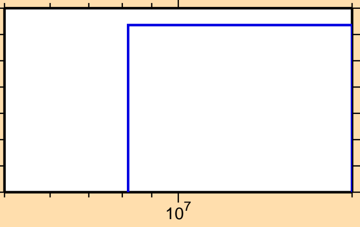
\sigma vs. E for ^{207}\text{Ra}(n,3n\alpha)
