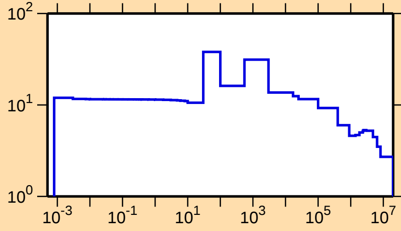
\sigma vs. E for ^{214}\text{Ra}(n,\text{el.})
