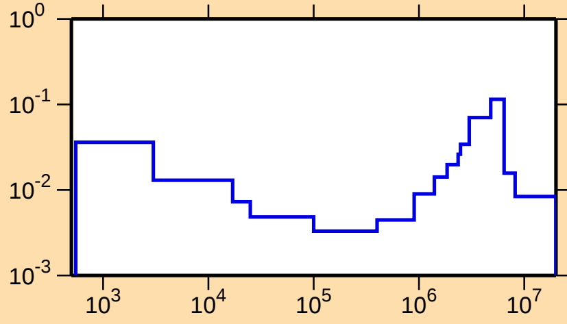
\sigma vs. E for ^{214}\text{Ra}(n,\alpha)
