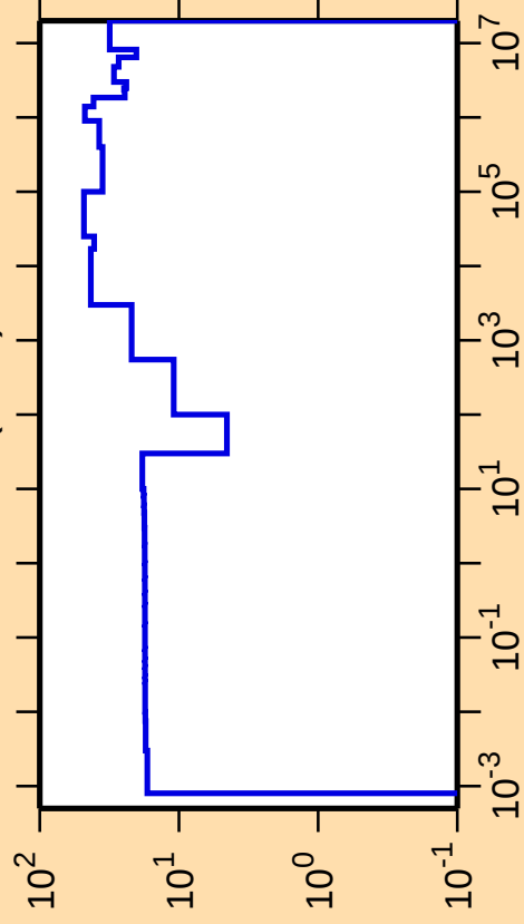
\Delta\sigma/\sigma vs. E for ^{214}\text{Ra}(n,\text{el.})
