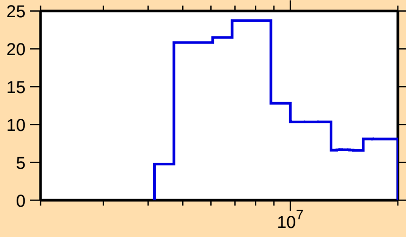
\Delta\sigma/\sigma vs. E for ^{229}\text{Ra}(n,\text{tot.})
