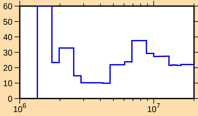
\Delta\sigma/\sigma vs. E for ^{229}\text{Ra}(n,n\text{cont.})
