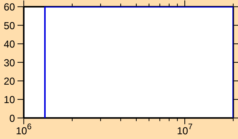
\Delta\sigma/\sigma vs. E for ^{229}\text{Ra}(n,\text{f})
