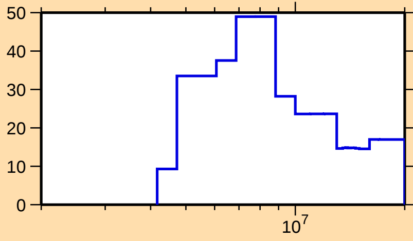
\Delta\sigma/\sigma vs. E for ^{229}\text{Ra}(n,\text{el.})
