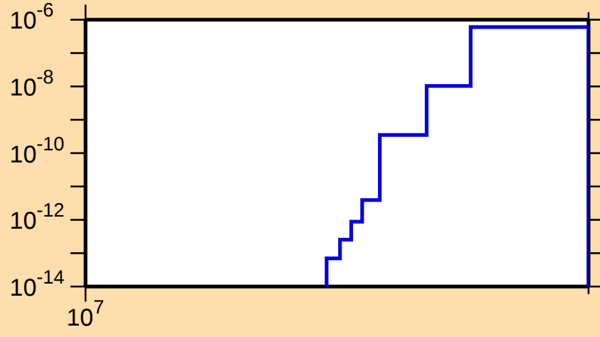
\sigma vs. E for ^{229}\text{Ra}(n,nt)
