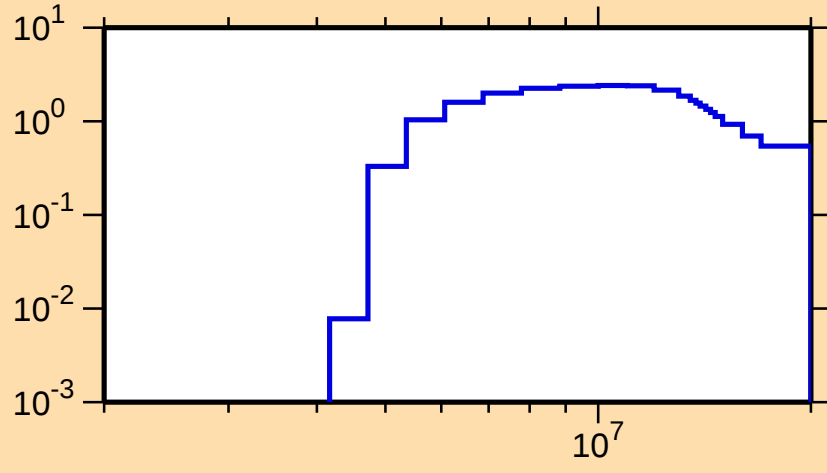
\sigma vs. E for ^{229}\text{Ra}(n,2n)
