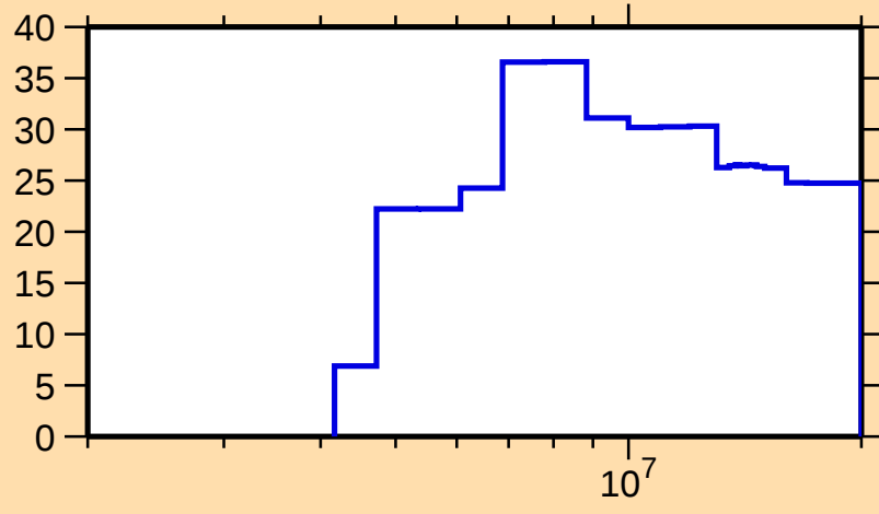
\Delta\sigma/\sigma vs. E for ^{229}\text{Ra}(n,\text{inel.})
