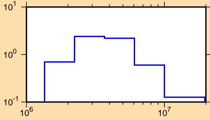
\sigma vs. E for ^{229}\text{Ra}(n,n\text{cont.})
