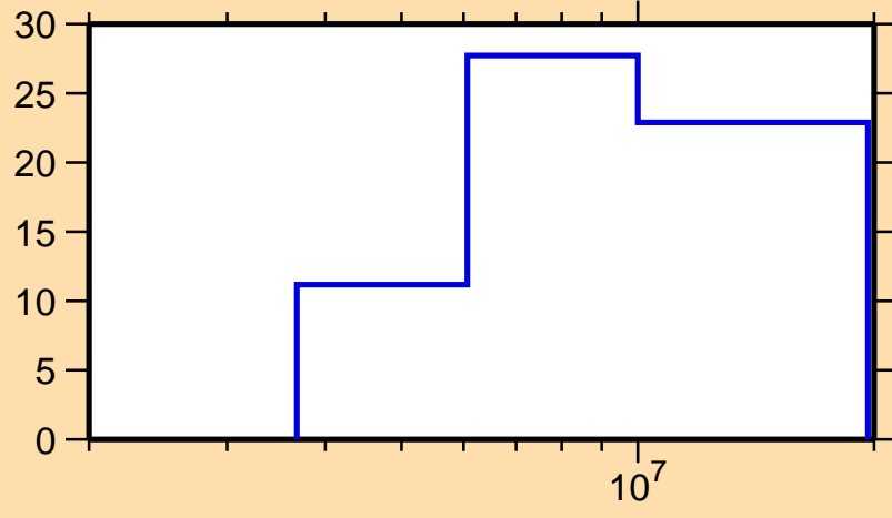
\Delta\sigma/\sigma vs. E for ^{229}\text{Ra}(n,n\text{cont.})
