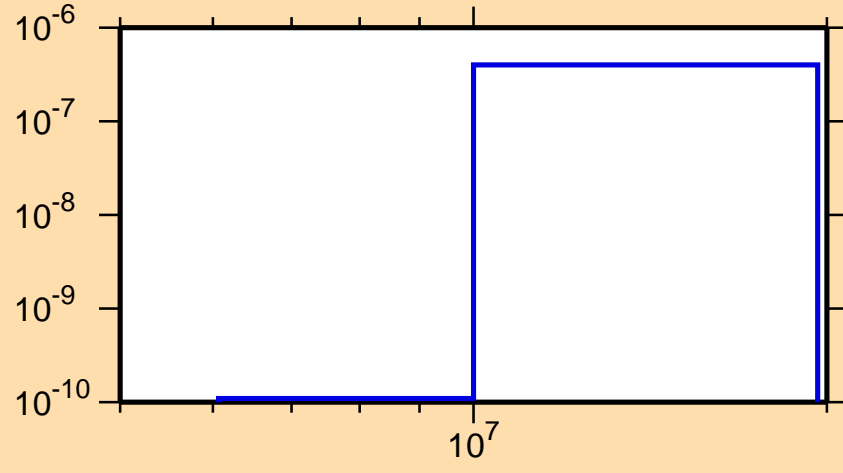
\sigma vs. E for ^{229}\text{Ra}(n,2n\alpha)
