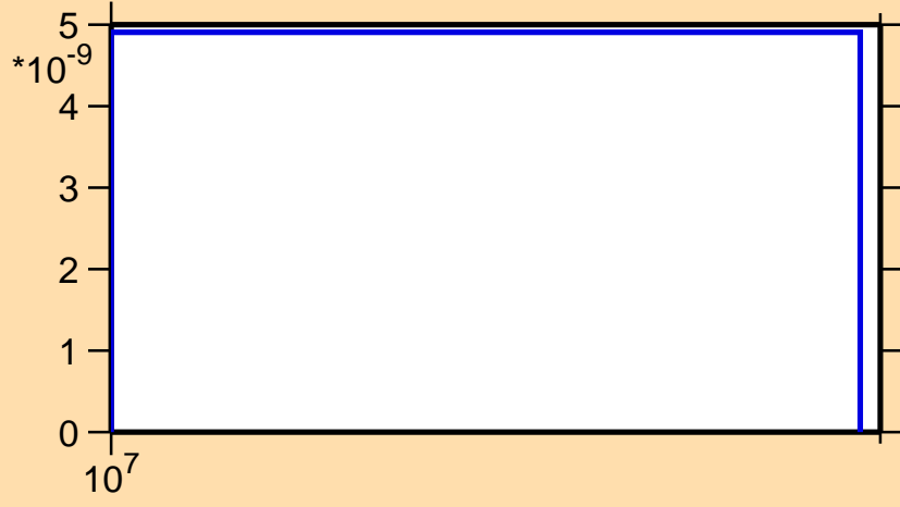
\sigma vs. E for ^{229}\text{Ra}(n,\text{nd})
