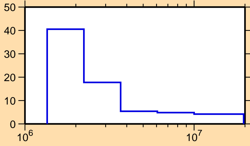
\Delta\sigma/\sigma vs. E for ^{229}\text{Ra}(n,\text{nonel.})
