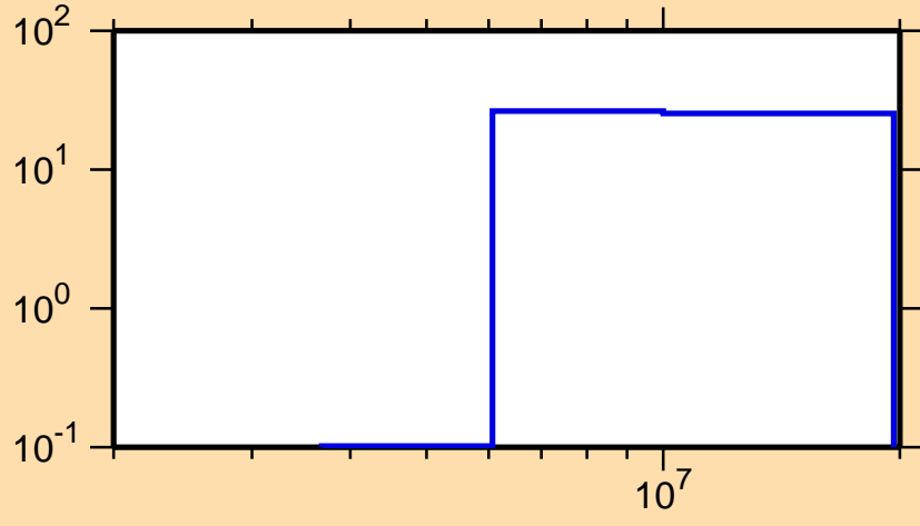
\Delta\sigma/\sigma vs. E for ^{229}\text{Ra}(n,p)
