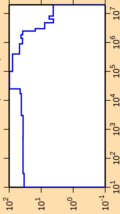
\Delta\sigma/\sigma vs. E for ^{229}\text{Ra}(n,\text{nonel.})
