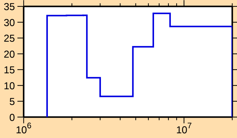
\Delta\sigma/\sigma vs. E for ^{229}\text{Ra}(n,\text{inel.})
