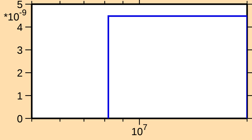
\sigma vs. E for ^{229}\text{Ra}(n,\text{nd})
