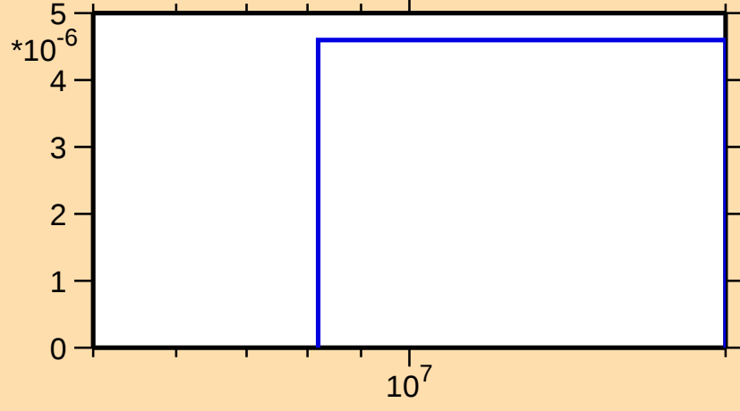
\sigma vs. E for ^{229}\text{Ra}(n,np)
