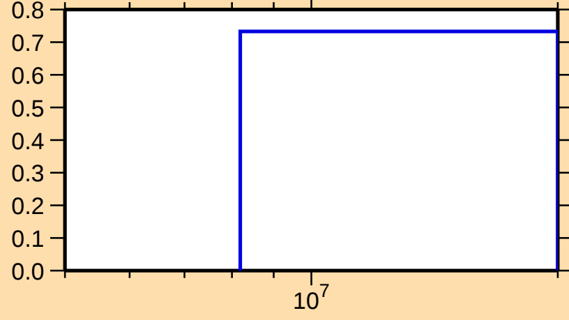
\sigma vs. E for ^{229}\text{Ra}(n,3n)
