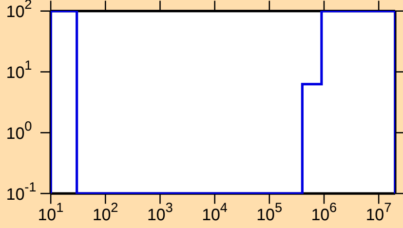
\Delta\sigma/\sigma vs. E for ^{229}\text{Ra}(n,f)
