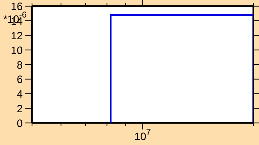
\sigma vs. E for ^{229}\text{Ra}(n,d)
