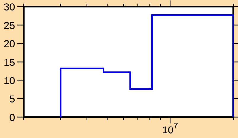
\Delta\sigma/\sigma vs. E for ^{229}\text{Ra}(n,2n)
