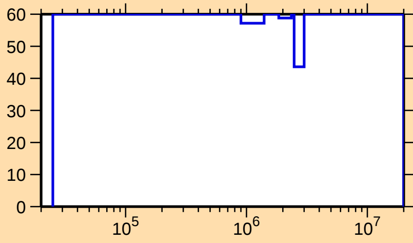
\Delta\sigma/\sigma vs. E for ^{229}\text{Ra}(n,n_1)
