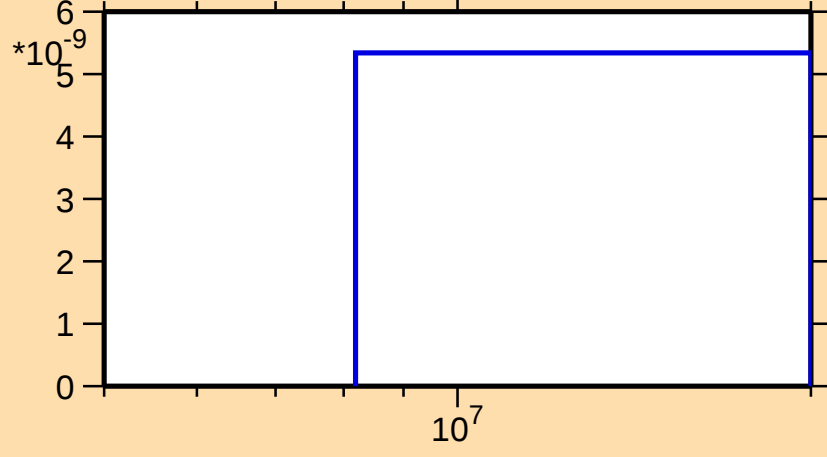
\sigma vs. E for ^{229}\text{Ra}(n,nt)
