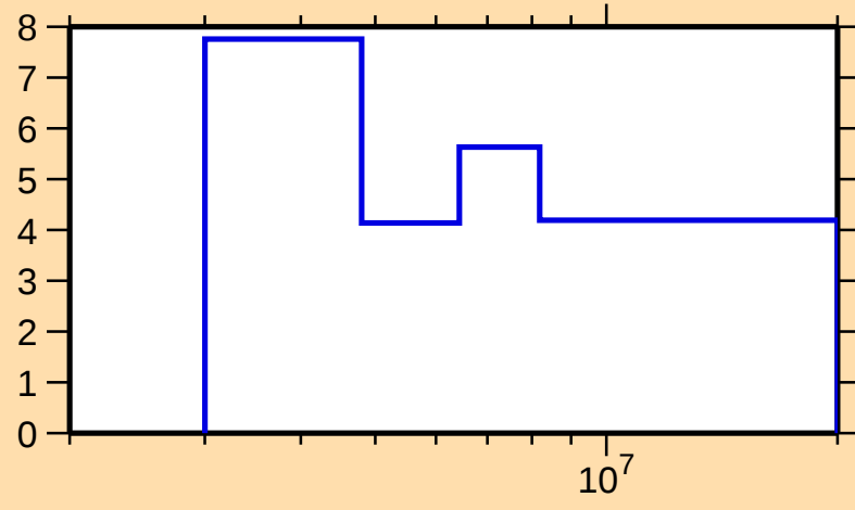
\Delta\sigma/\sigma vs. E for ^{229}\text{Ra}(n,\text{nonel.})
