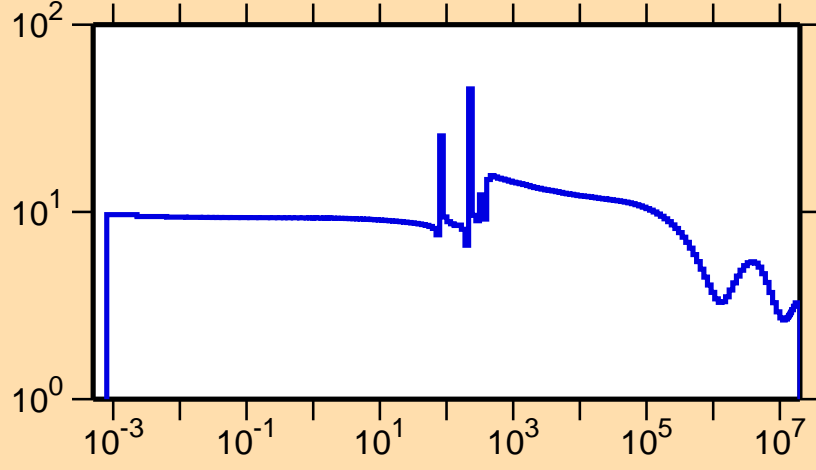
\sigma vs. E for ^{232}\text{Ra}(n,\text{el.})
