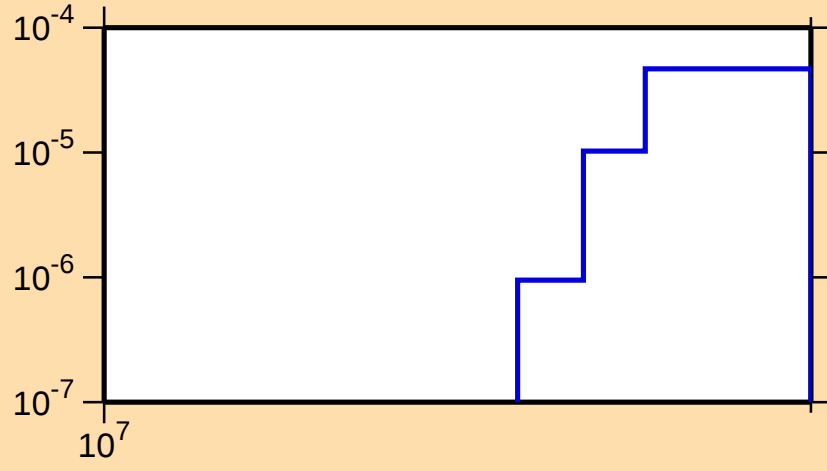
\sigma vs. E for ^{91}\text{Rh}(n,2n)
