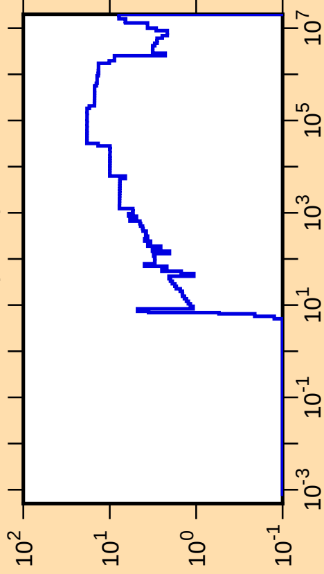
\Delta\sigma/\sigma vs. E for ^{91}\text{Rh}(n,\text{tot.})
