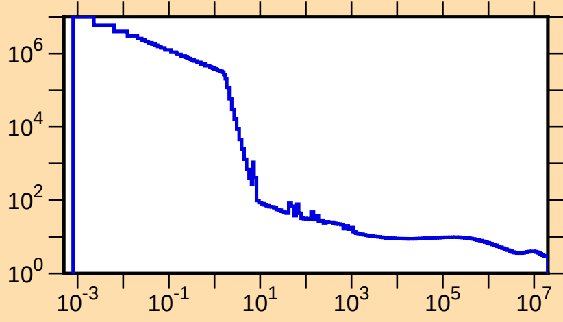
\sigma vs. E for ^{91}\text{Rh}(n,\text{tot.})
