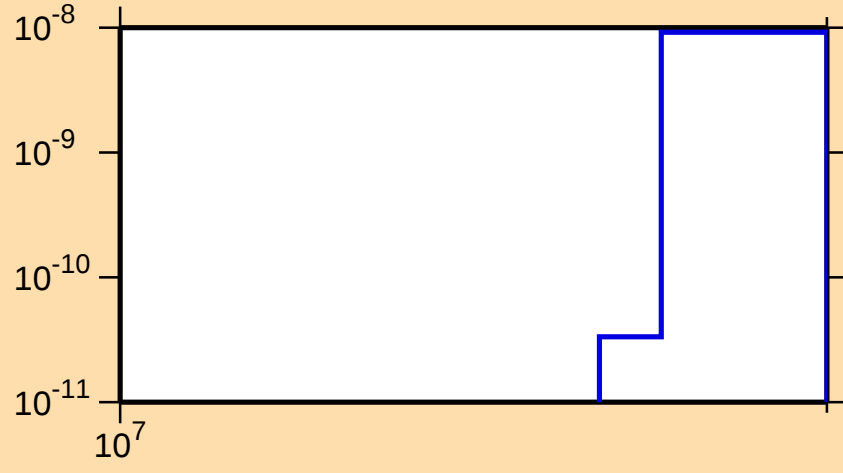
\sigma vs. E for ^{91}\text{Rh}(n,\text{nd})
