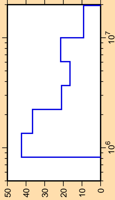
\Delta\sigma/\sigma vs. E for ^{91}\text{Rh}(n,n_3)
