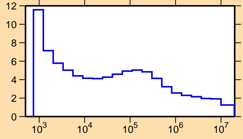
\sigma vs. E for ^{91}\text{Rh}(n,\text{nonel.})
