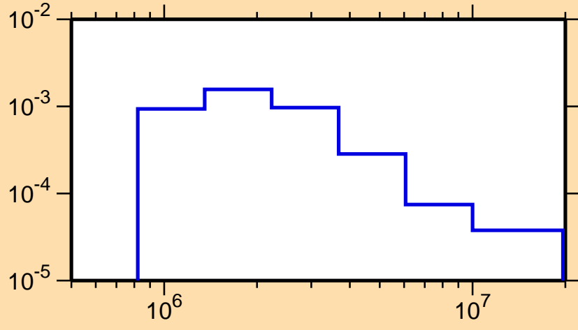
\sigma vs. E for ^{91}\text{Rh}(n,n_3)
