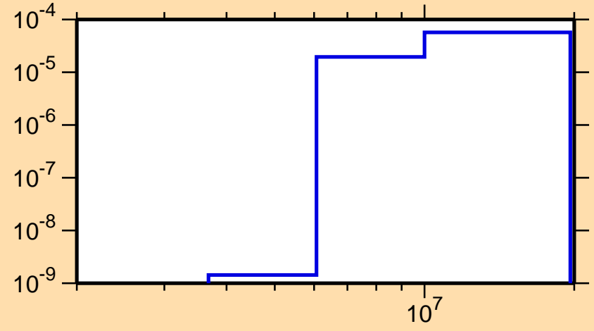
\sigma vs. E for ^{91}\text{Rh}(n,n\text{cont.})
