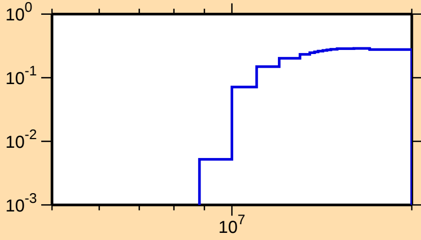
\sigma vs. E for ^{96}\text{Rh}(n,2n)
