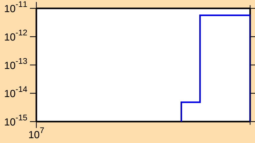
\sigma vs. E for ^{96}\text{Rh}(n,2n\alpha)
