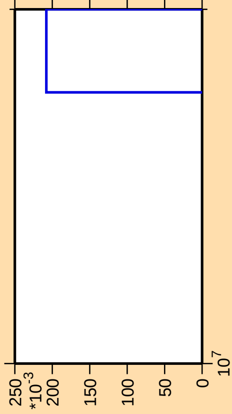
\Delta\sigma/\sigma vs. E for ^{96}\text{Rh}(n,nt)
