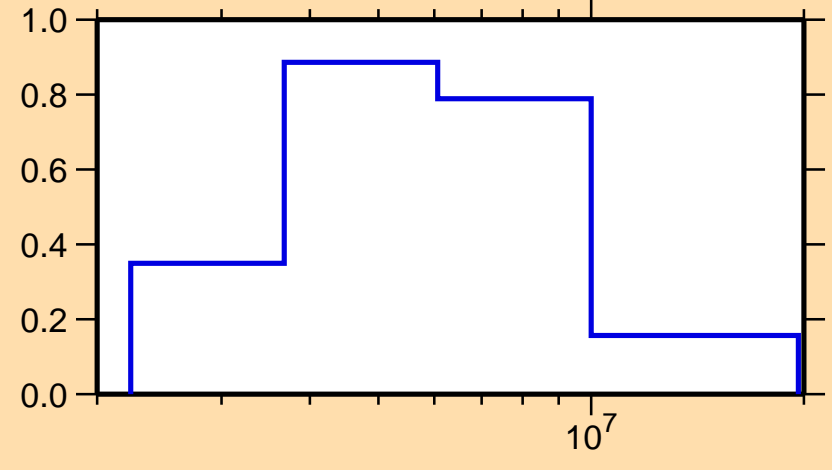
\sigma vs. E for ^{96}\text{Rh}(n,n\text{cont.})
