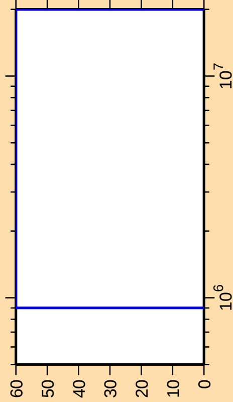
\Delta\sigma/\sigma vs. E for ^{96}\text{Rh}(n,p\alpha)
