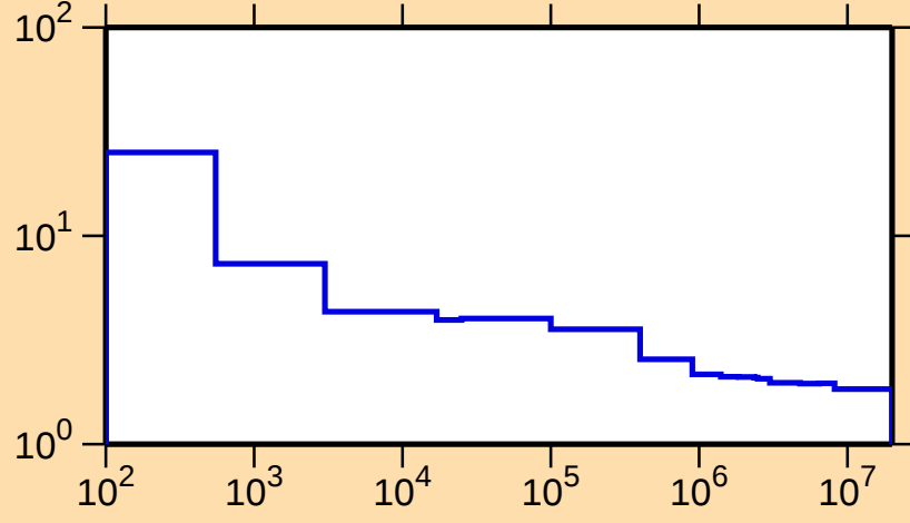
\sigma vs. E for ^{96}\text{Rh}(n,\text{nonel.})
