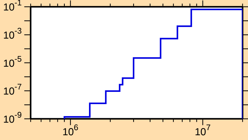
\sigma vs. E for ^{96}\text{Rh}(n,p\alpha)
