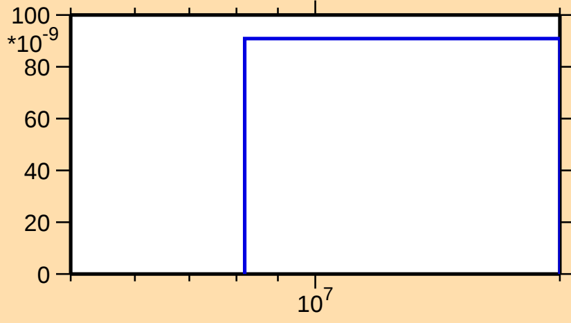
\sigma vs. E for ^{96}\text{Rh}(\text{mt } 45)
