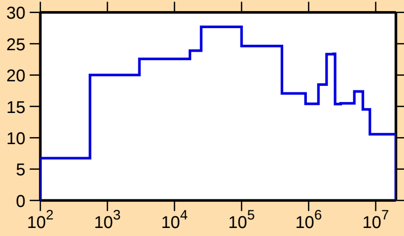
\Delta\sigma/\sigma vs. E for ^{96}\text{Rh}(n,\text{el.})
