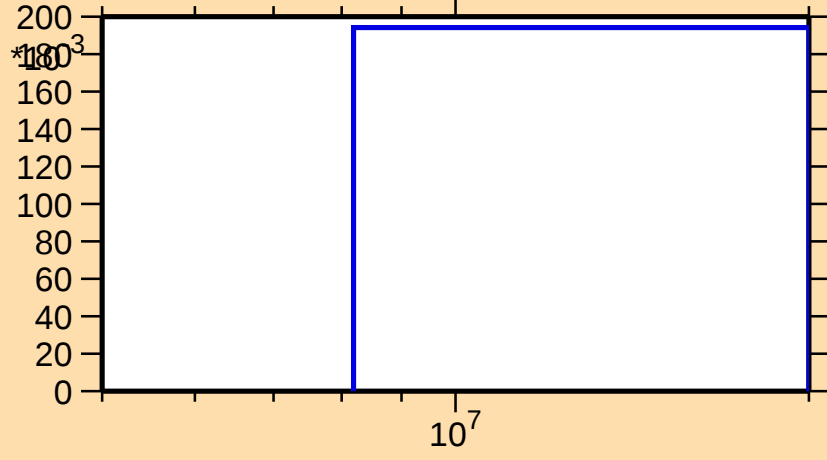
\sigma vs. E for ^{96}\text{Rh}(n,2n)
