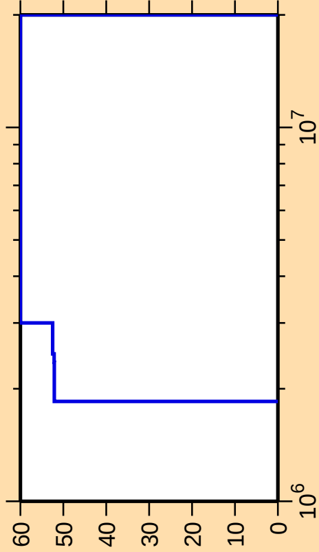
\Delta\sigma/\sigma vs. E for ^{96}\text{Rh}(n,\alpha)
