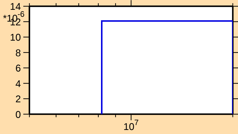
\sigma vs. E for ^{96}\text{Rh}(n,\text{nd})
