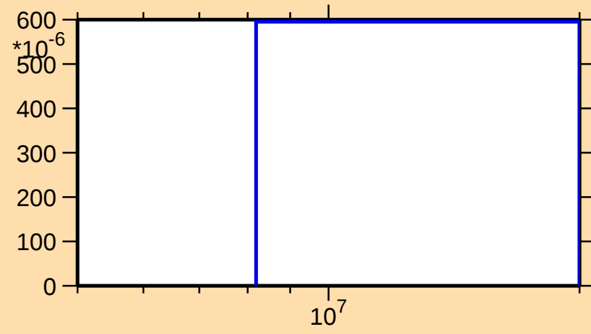
\sigma vs. E for ^{96}\text{Rh}(n,2np)
