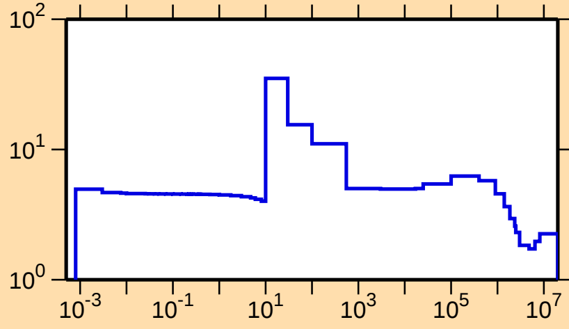
\sigma vs. E for ^{96}\text{Rh}(n,\text{el.})
