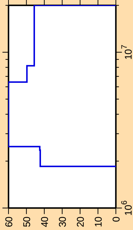
\Delta\sigma/\sigma vs. E for ^{96}\text{Rh}(n,p)
