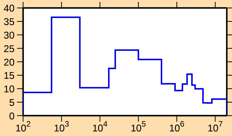
\Delta\sigma/\sigma vs. E for ^{96}\text{Rh}(n,\text{tot.})
