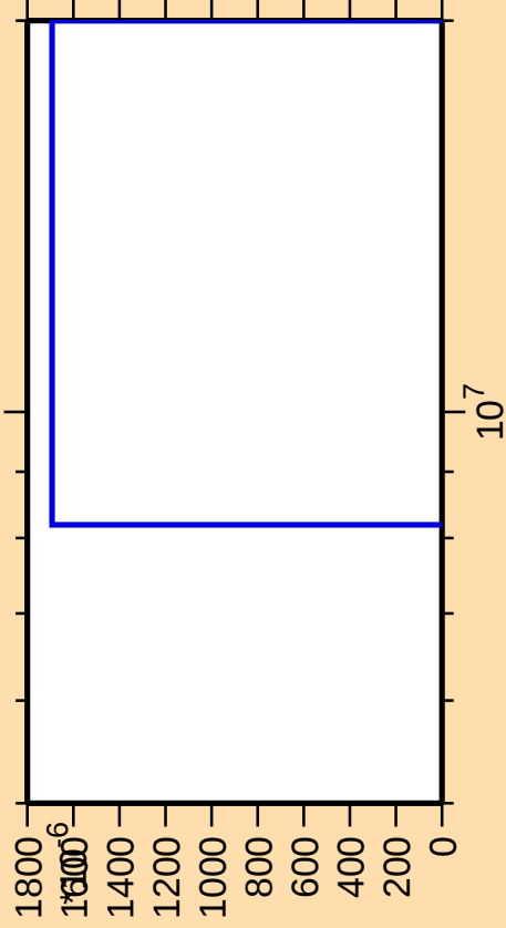
\Delta\sigma/\sigma vs. E for ^{96}\text{Rh}(n,nt)
