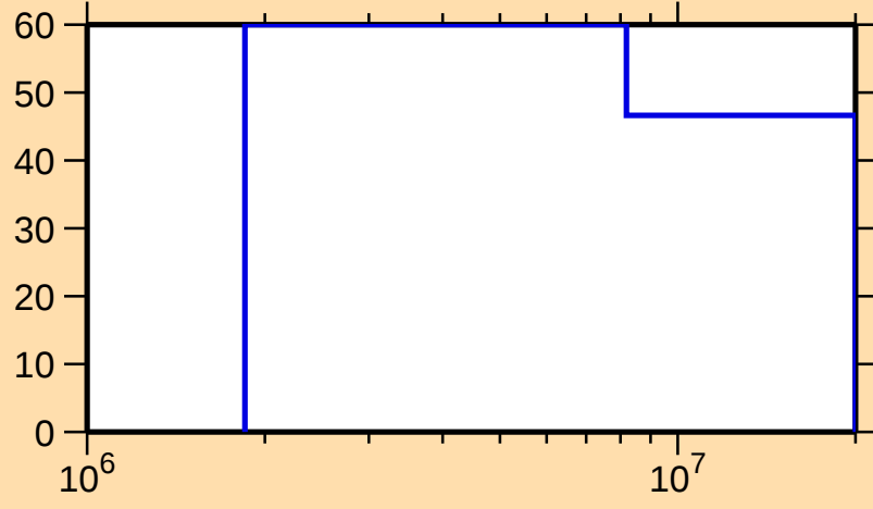
\Delta\sigma/\sigma vs. E for ^{96}\text{Rh}(n,n\text{cont.})
