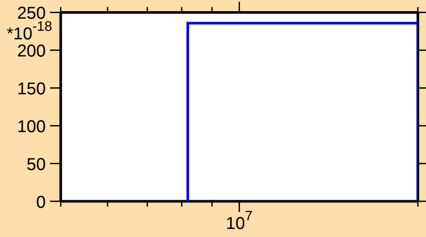
\sigma vs. E for ^{96}\text{Rh}(n,nt)
