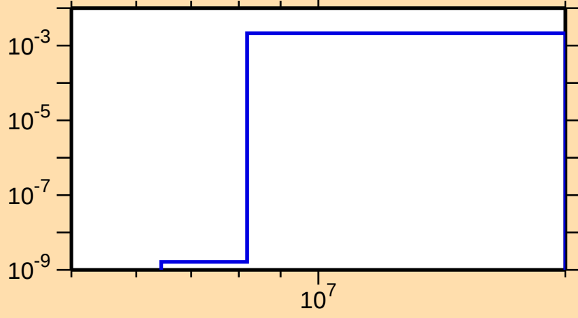
\sigma vs. E for ^{96}\text{Rh}(n,n\alpha)
