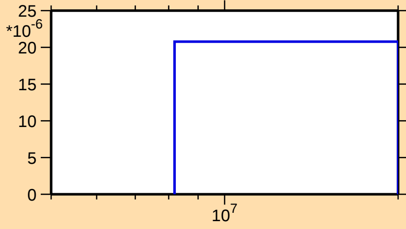
\sigma vs. E for ^{96}\text{Rh}(n,\text{pd})
