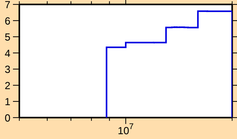
\Delta\sigma/\sigma vs. E for ^{103}\text{Rh}(n,\text{tot.})
