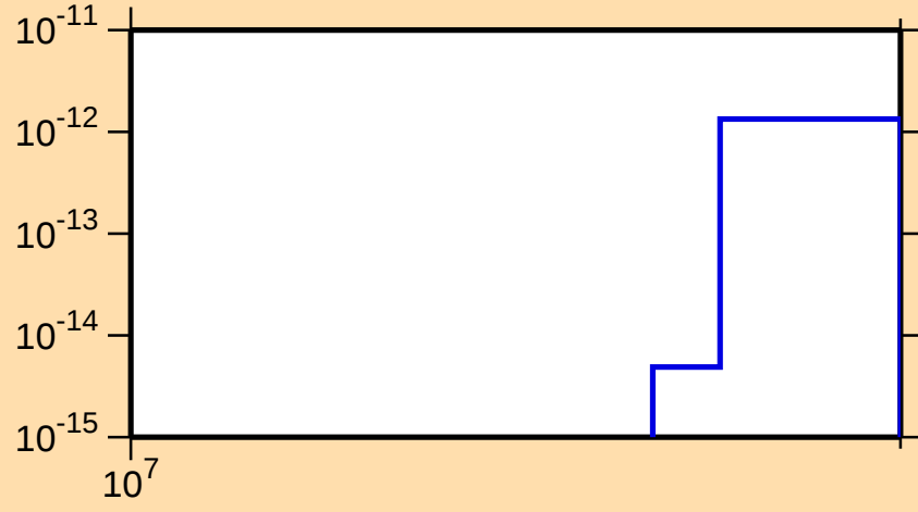
\sigma vs. E for ^{103}\text{Rh}(\text{mt } 45)
