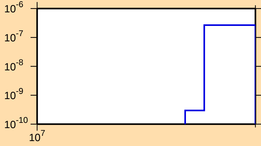
\sigma vs. E for ^{103}\text{Rh}(n,\text{nt})
