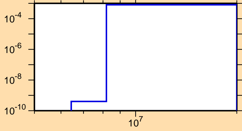
\sigma vs. E for ^{103}\text{Rh}(n,n\alpha)
