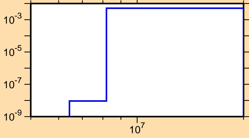
\sigma vs. E for ^{103}\text{Rh}(n,np)
