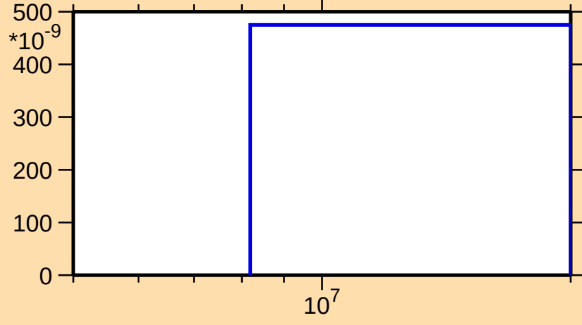
\sigma vs. E for ^{230}\text{Rn}(n,d)
