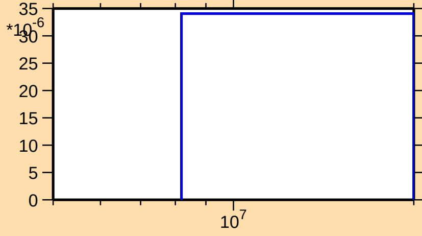
\sigma vs. E for ^{230}\text{Rn}(n,p)
