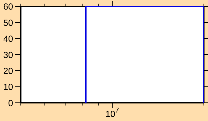
\Delta\sigma/\sigma vs. E for ^{230}\text{Rn}(n,n\text{cont.})
