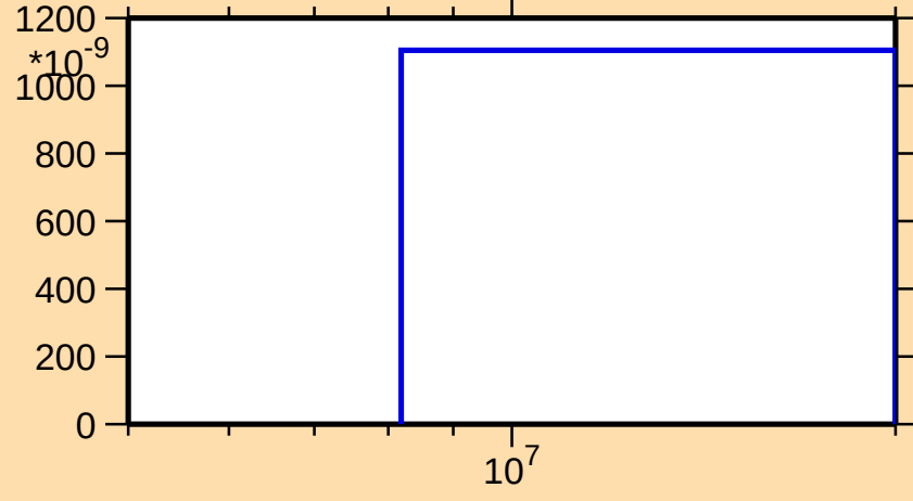
\sigma vs. E for ^{230}\text{Rn}(n,np)
