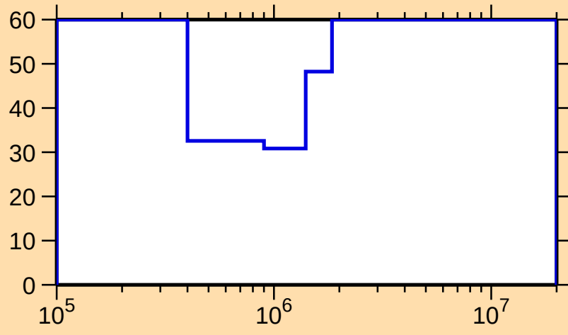
\Delta\sigma/\sigma vs. E for ^{230}\text{Rn}(n,n_1)
