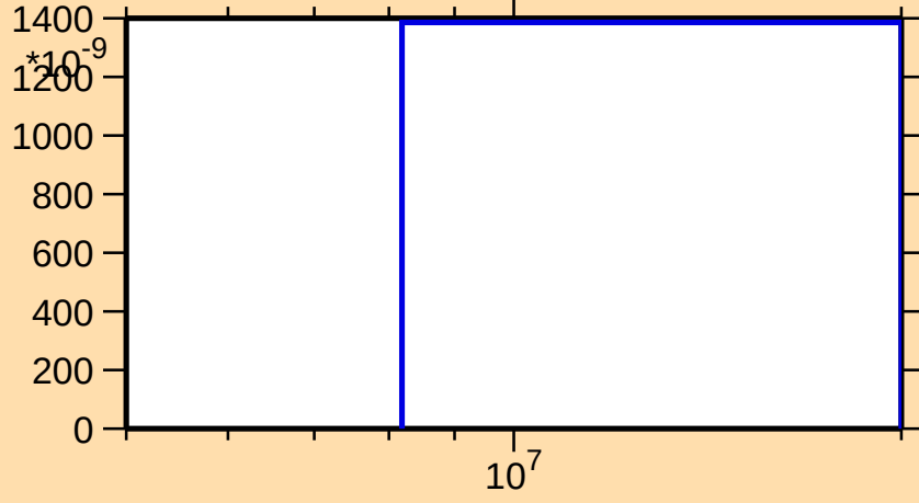
\sigma vs. E for ^{230}\text{Rn}(n,t)
