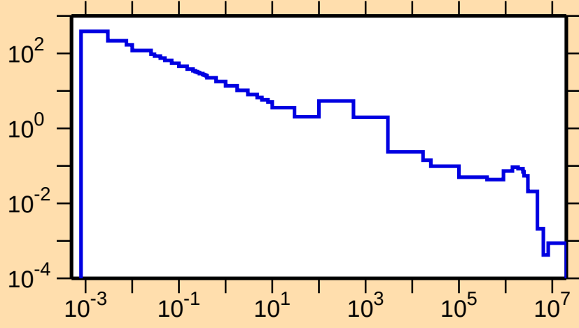
\sigma vs. E for ^{230}\text{Rn}(n,\gamma)
