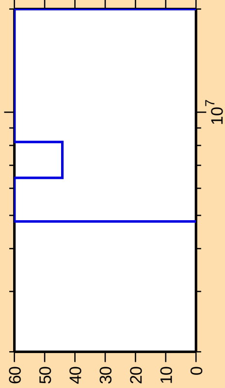
\Delta\sigma/\sigma vs. E for ^{230}\text{Rn}(n,2n)
