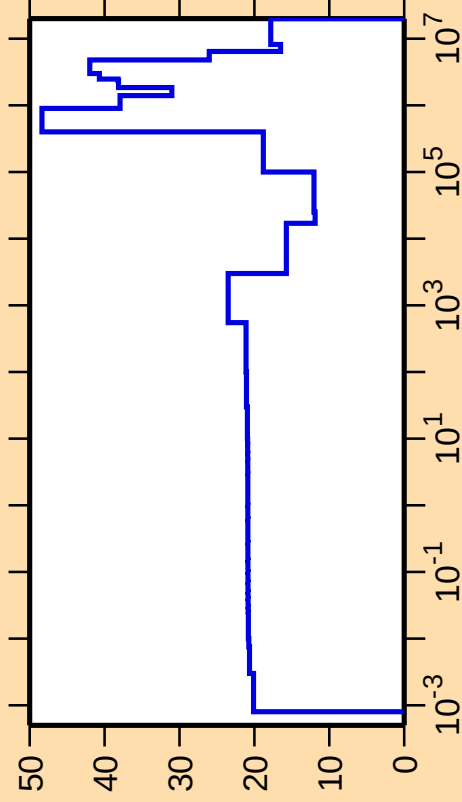
\Delta\sigma/\sigma vs. E for ^{230}\text{Rn}(n,\text{el.})
