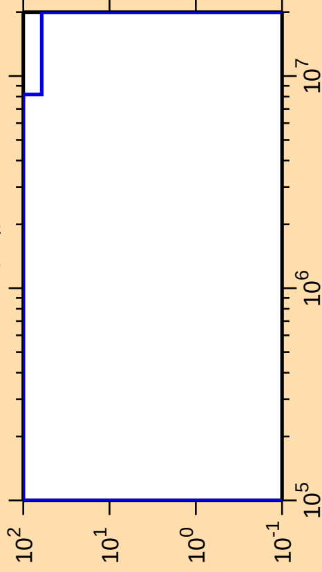
\Delta\sigma/\sigma vs. E for ^{230}\text{Rn}(n,\gamma)
