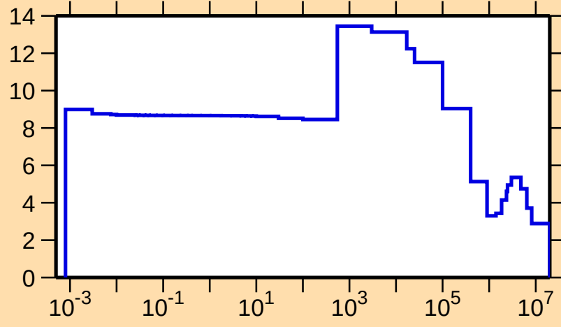
\sigma vs. E for ^{230}\text{Rn}(n,\text{el.})
