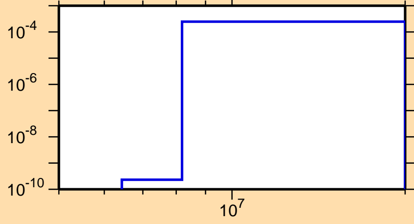
\sigma vs. E for ^{102}\text{Ru}(n,n\alpha)
