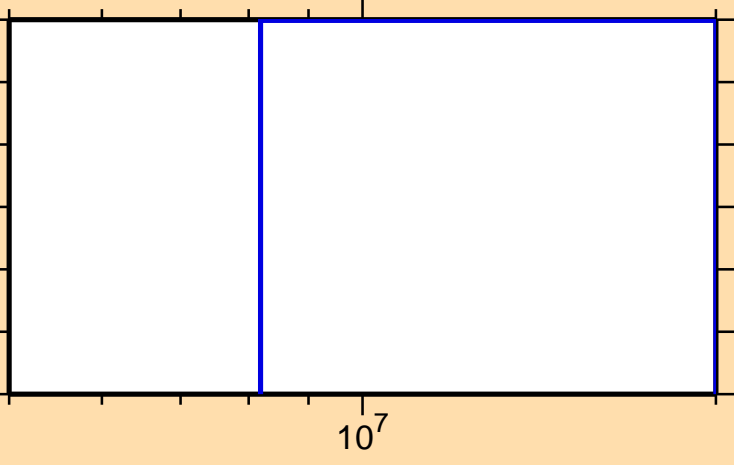
\sigma vs. E for ^{102}\text{Ru}(n,t)
