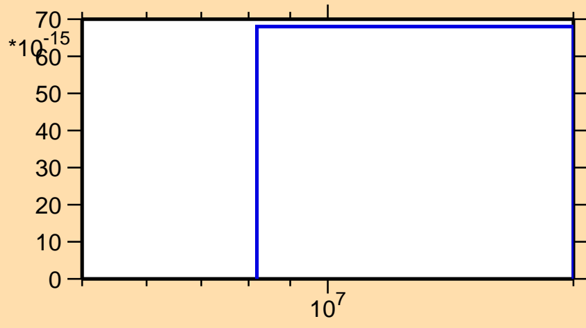
\sigma vs. E for ^{102}\text{Ru}(n,p\alpha)
