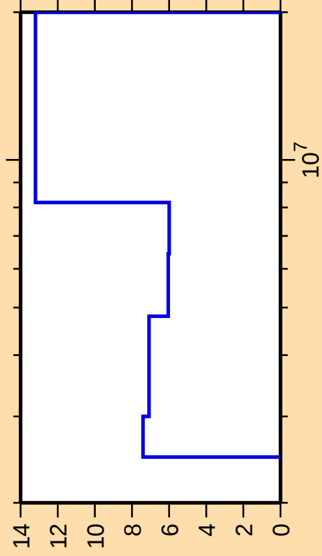
\Delta\sigma/\sigma vs. E for ^{76}\text{Se}(\text{n},\text{ncont.})
