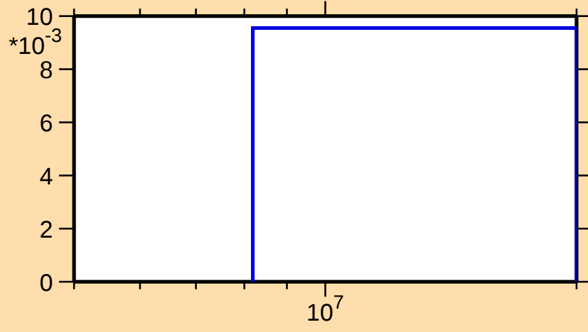
\sigma vs. E for ^{76}\text{Se}(n,np)
