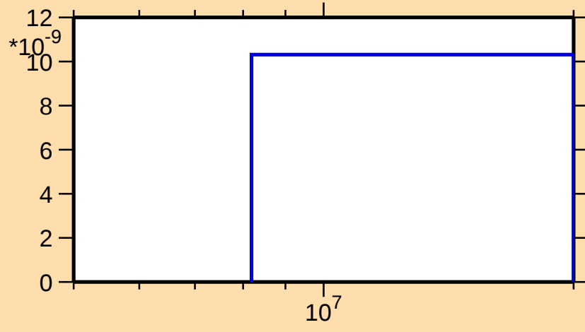
\sigma vs. E for ^{76}\text{Se}(n,3n)
