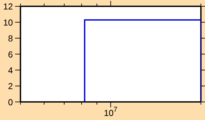
\Delta\sigma/\sigma vs. E for ^{76}\text{Se}(n,\text{inel.})
