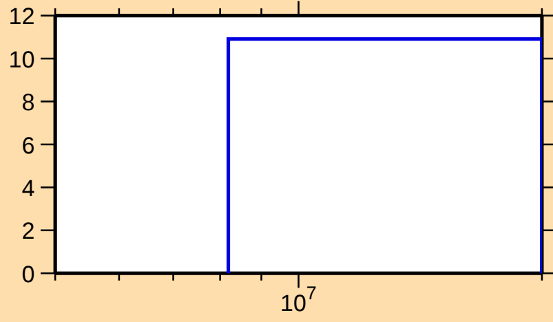
\Delta\sigma/\sigma vs. E for ^{76}\text{Se}(n,\text{el.})
