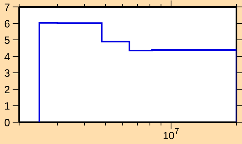
\Delta\sigma/\sigma vs. E for ^{76}\text{Se}(\text{n},\text{nonel.})
