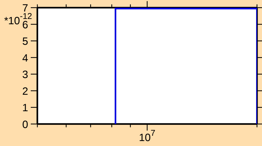
\sigma vs. E for ^{76}\text{Se}(n,\text{nd})
