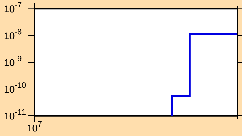
\sigma vs. E for ^{161}\text{Ta}(n,\text{nt})
