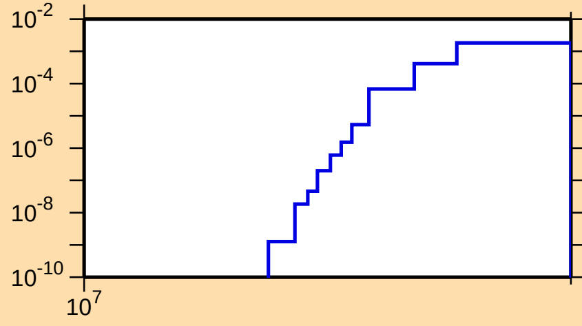
\sigma vs. E for ^{161}\text{Ta}(n,2np)
