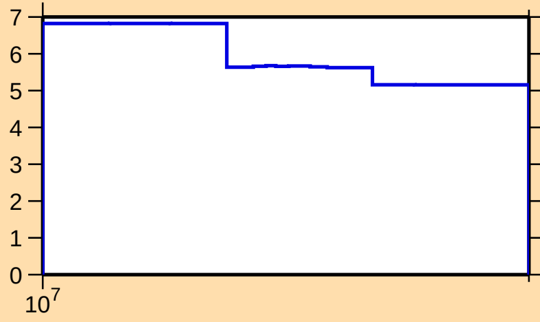
\Delta\sigma/\sigma vs. E for ^{161}\text{Ta}(n,\text{nonel.})
