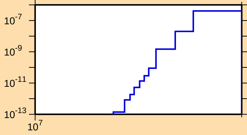
\sigma vs. E for ^{161}\text{Ta}(n,\text{pt})
