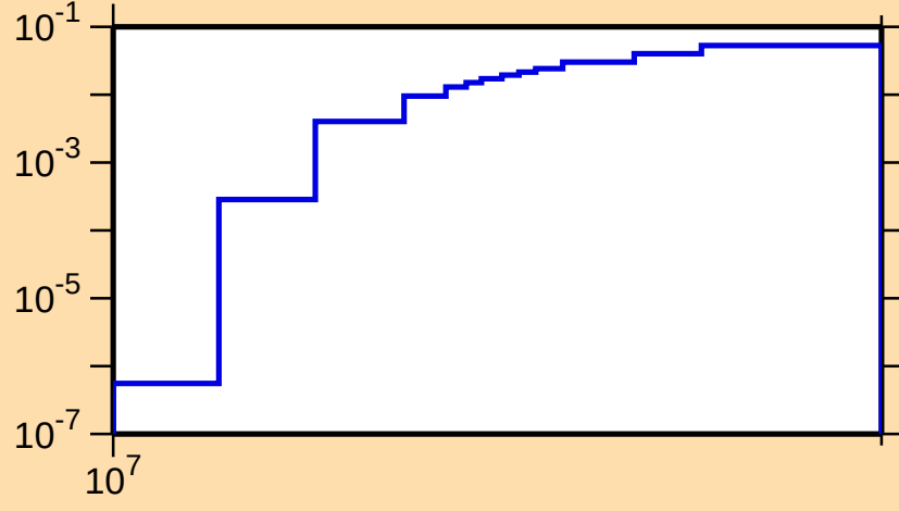
\sigma vs. E for ^{161}\text{Ta}(n,2n)
