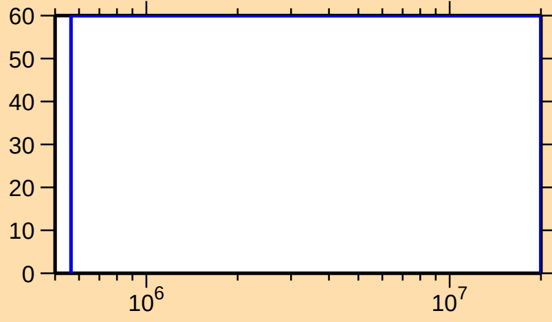
\Delta\sigma/\sigma vs. E for ^{161}\text{Ta}(n,n\text{cont.})
