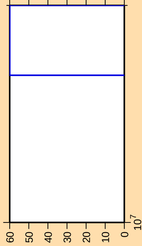
\Delta\sigma/\sigma vs. E for ^{161}\text{Ta}(n,\text{nt})
