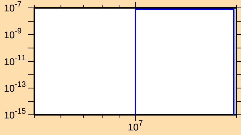
\sigma vs. E for ^{161}\text{Ta}(n,\text{nd})
