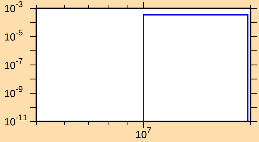
\sigma vs. E for ^{161}\text{Ta}(n,2n\alpha)
