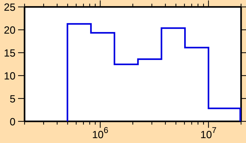
\Delta\sigma/\sigma vs. E for ^{161}\text{Ta}(n,\text{tot.})
