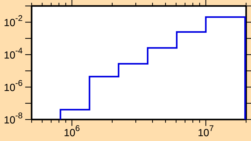
\sigma vs. E for ^{161}\text{Ta}(n,n\alpha)
