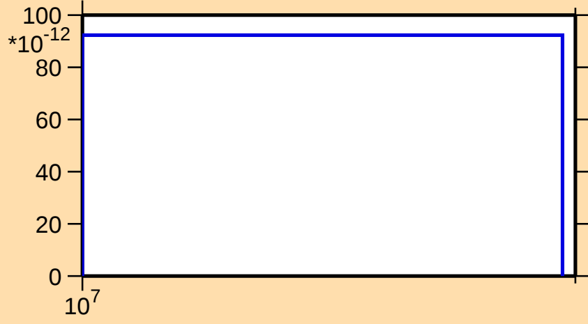
\sigma vs. E for ^{161}\text{Ta}(n,\text{nt})
