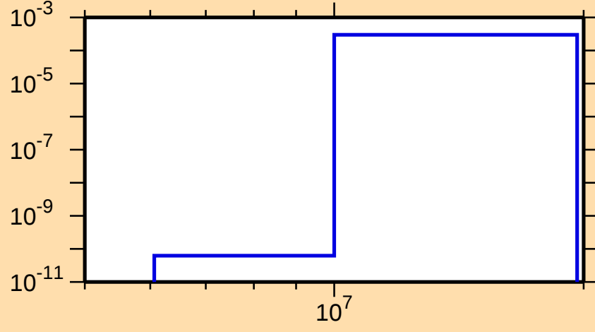
\sigma vs. E for ^{161}\text{Ta}(n,t)
